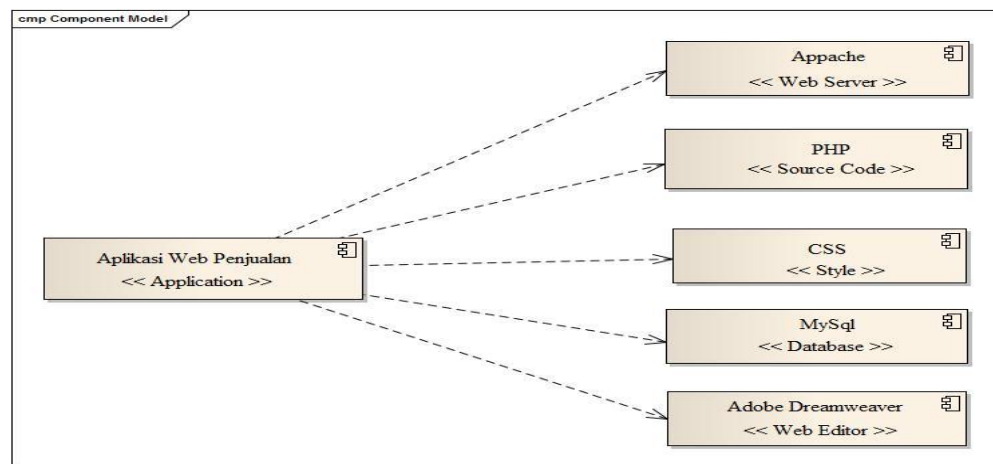
Gambar IV.9 Component Diagram
