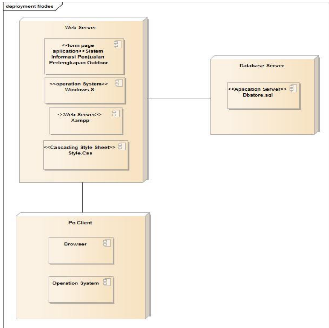
Gambar IV.10 Deployment Diagram
