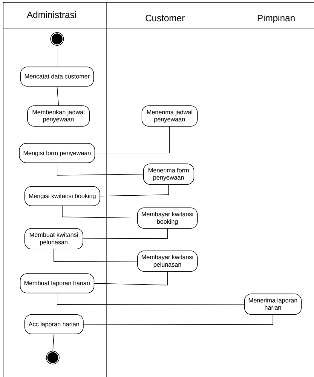
Gambar : III.2 Activity Diagram Berjalan
