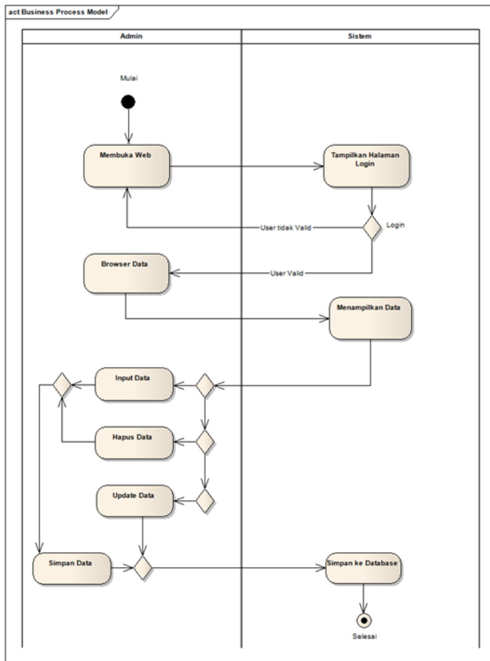
Gambar IV.4 Activity Diagram Admin Mengelola Data
