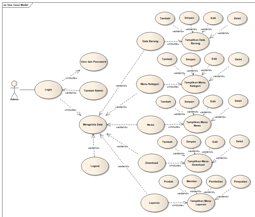
Gambar IV.2 Use Case halaman admin
