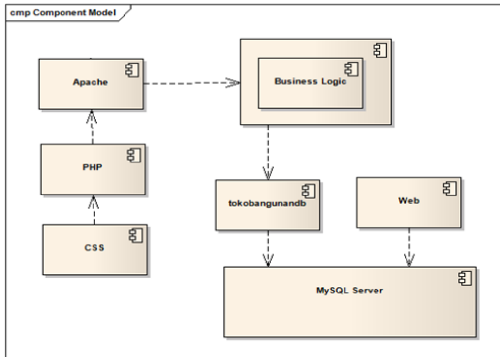
Gambar IV.6 Component Diagram
