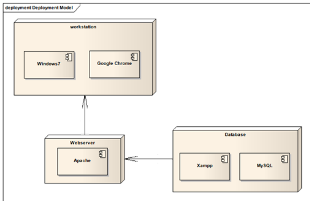
Gambar IV.7 Deployment Diagram
