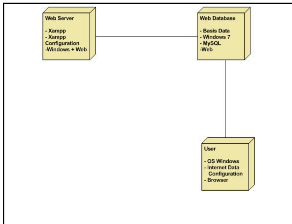
Gambar IV. 9 Deployment Diagram
