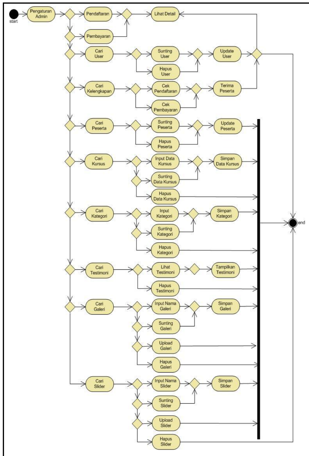
Gambar IV. 5 Activity Diagram Halaman Admin
