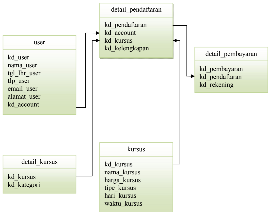
Gambar IV. 7 Logical Record Structure Pendaftaran Online
