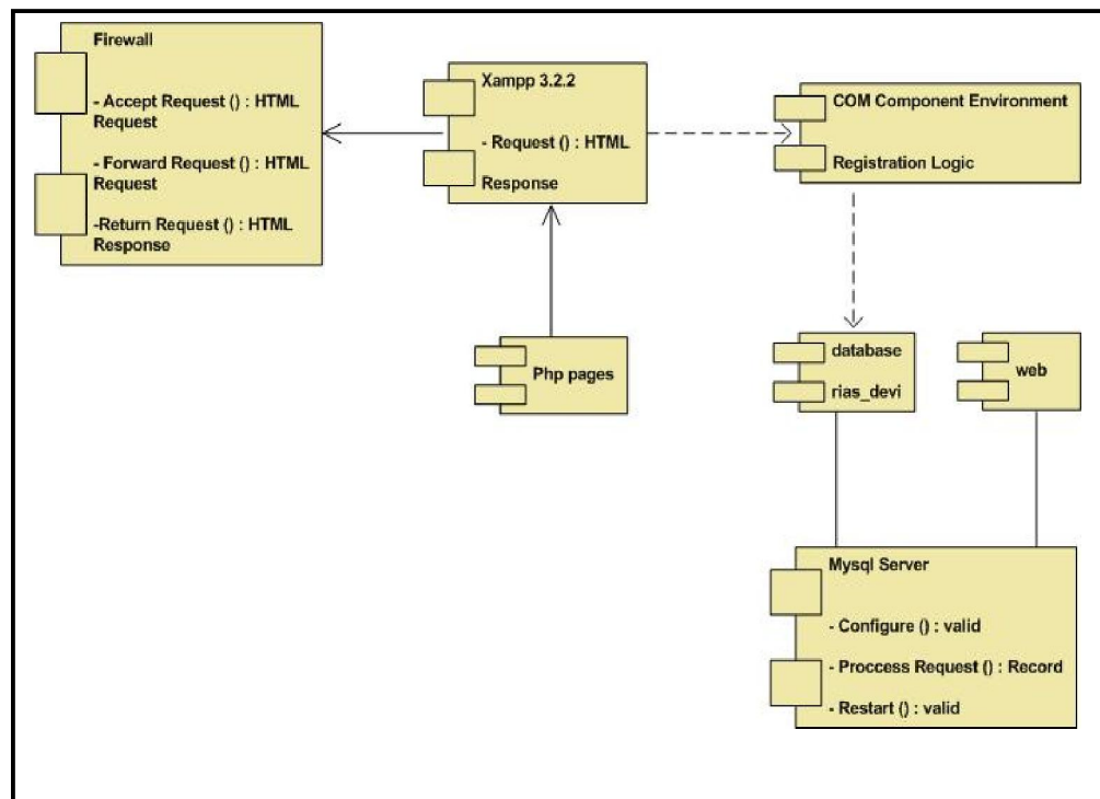
Gambar IV. 8 Component Diagram
