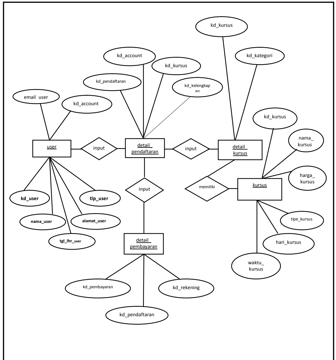
Gambar IV. 6 Entity Relationship Diagram Pendaftaran Online
