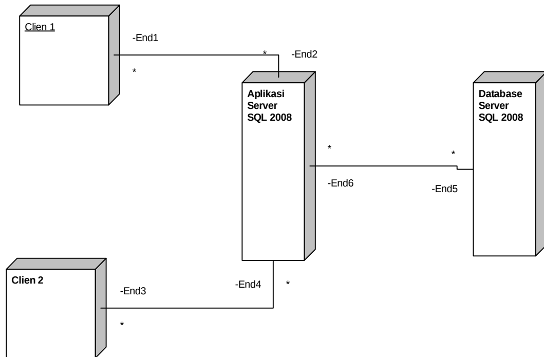
Gambar IV.13. Deployment Diagram
