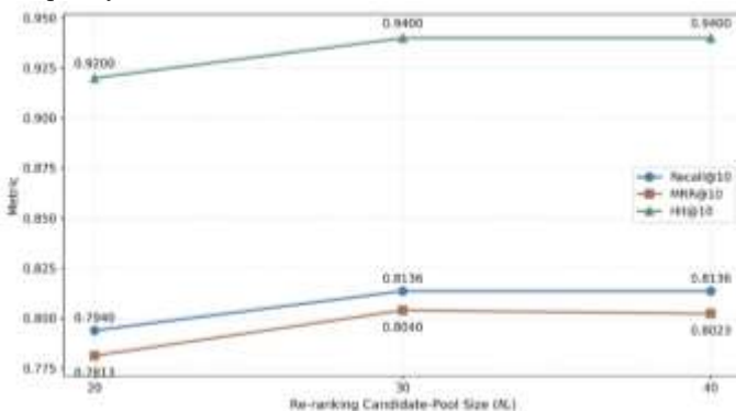
Fig. 3. Effect of the re-ranking candidate-pool size ( N_r ) on Recall@10, MRR@10, and Hit@10 Performance improves from 20 to 30 candidates and plateaus at 40, supporting the use of ( N_r=30 ).
