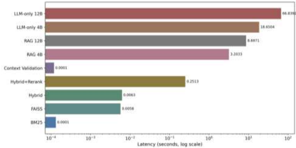
Fig. 5. Mean latency across retrieval stages and end-to-end configurations
