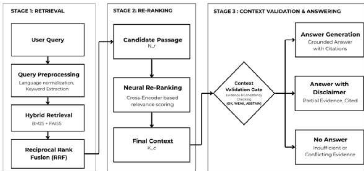
Fig. 1. Architecture of the proposed multi-stage RAG pipeline
