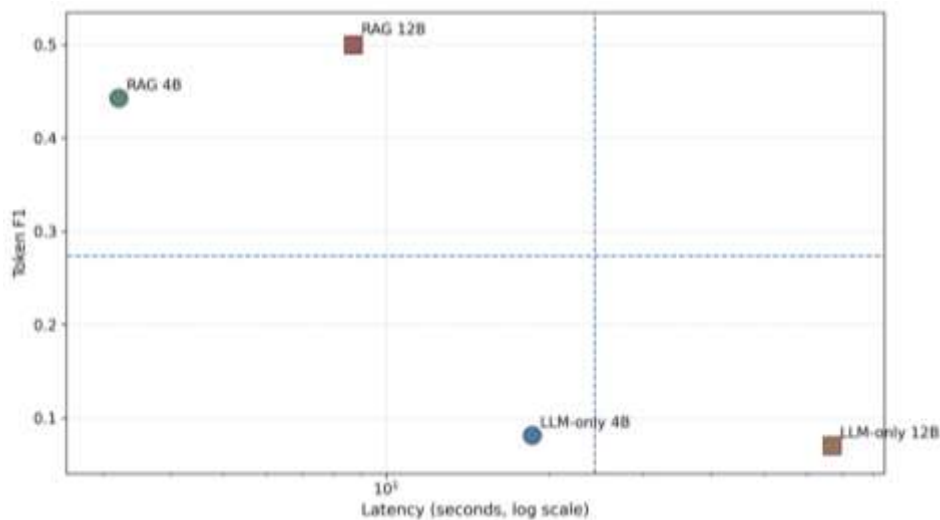
Fig. 6. Token F1–latency trade-off across RAG and LLM-only configurations
