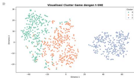
Figure 9. Visualization of Game Clusters with t-SNE
