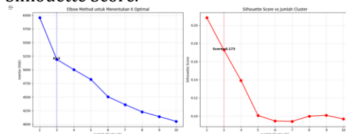
Figure 6. Elbow and Silhouette Score for Determining K
