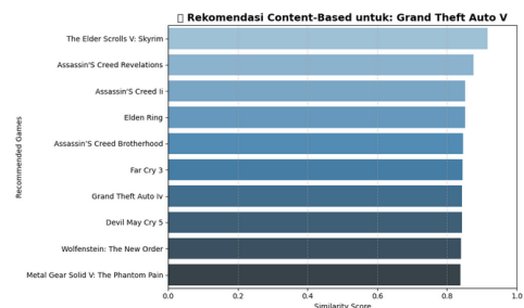
Figure 11. Visualization of Content-based Filtering Recommendations.
