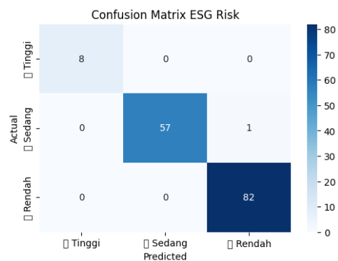
Figure 5. Confusion Matrix Random Forest
