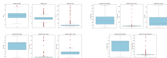
Figure 3. Boxplot Visualization
