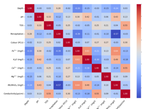
Figure 2. Heatmap Visualization
