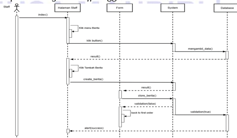
Gambar IV.32 Sequence Diagram Staff Unggah Berita
