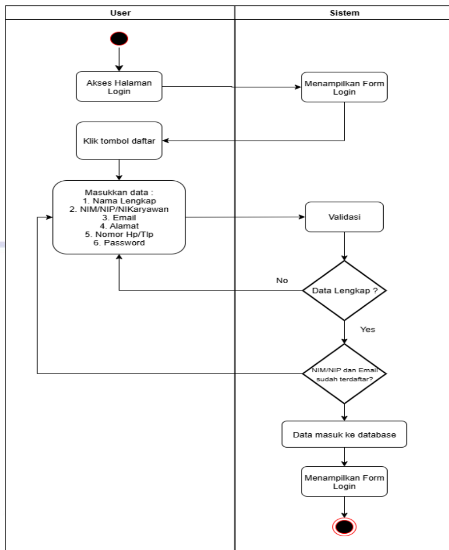
Gambar IV.2 Activity Diagram Register
