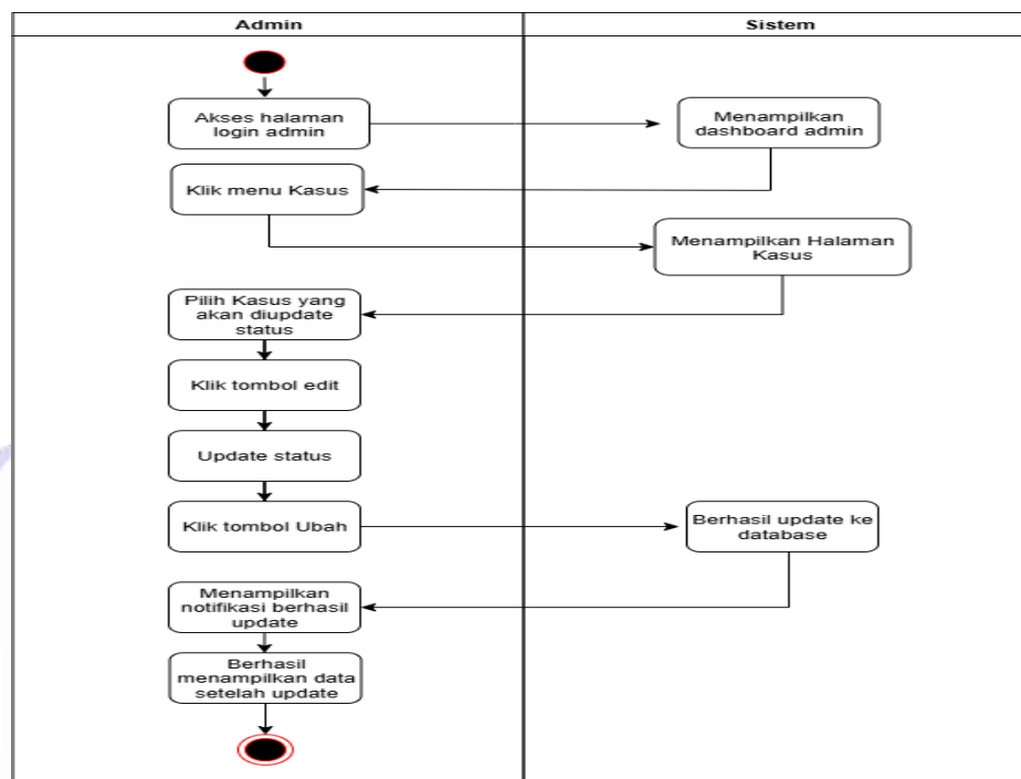
Gambar IV.8 Activity Diagram Update Status Pengaduan
