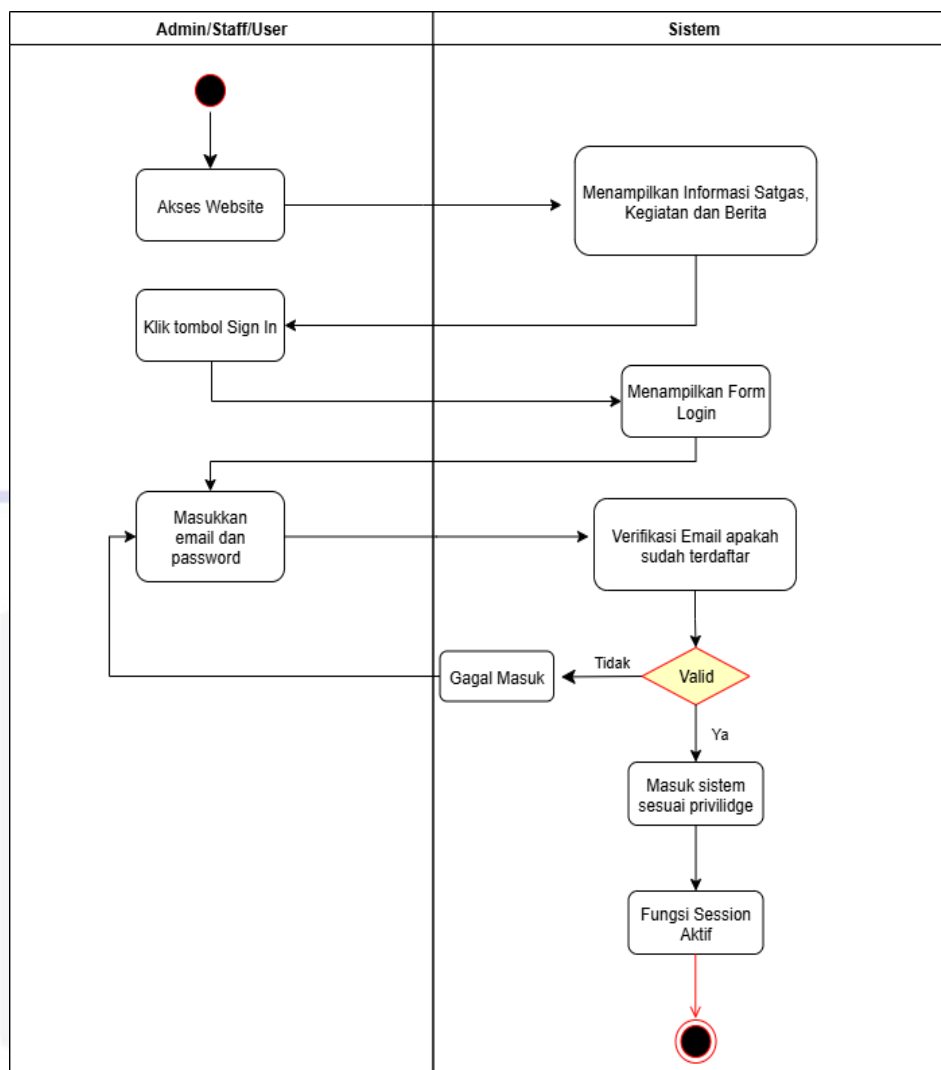
Gambar IV.3 Activity Diagram Login
