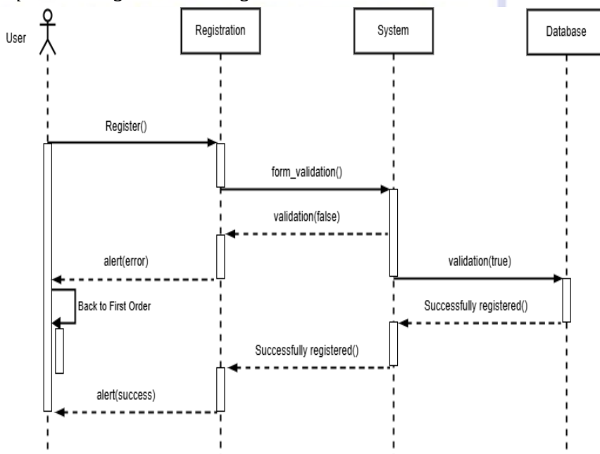
Gambar IV.15 Sequence Diagram User Register
