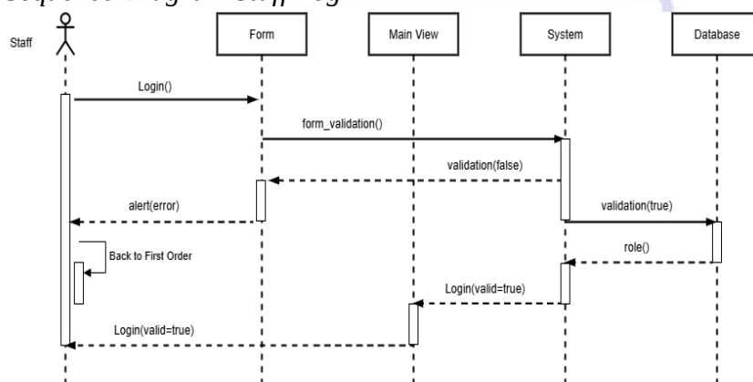
Gambar IV. 28 Sequence Diagram Staff Login
