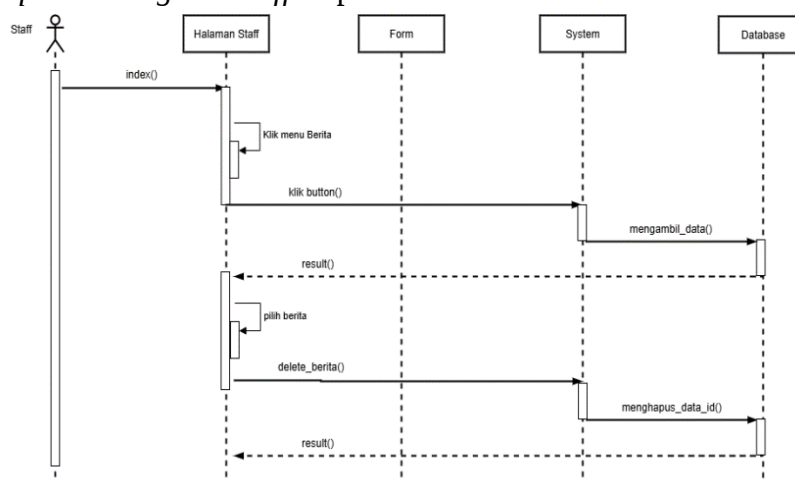
Gambar IV.33 Sequence Diagram Staff Hapus Berita
