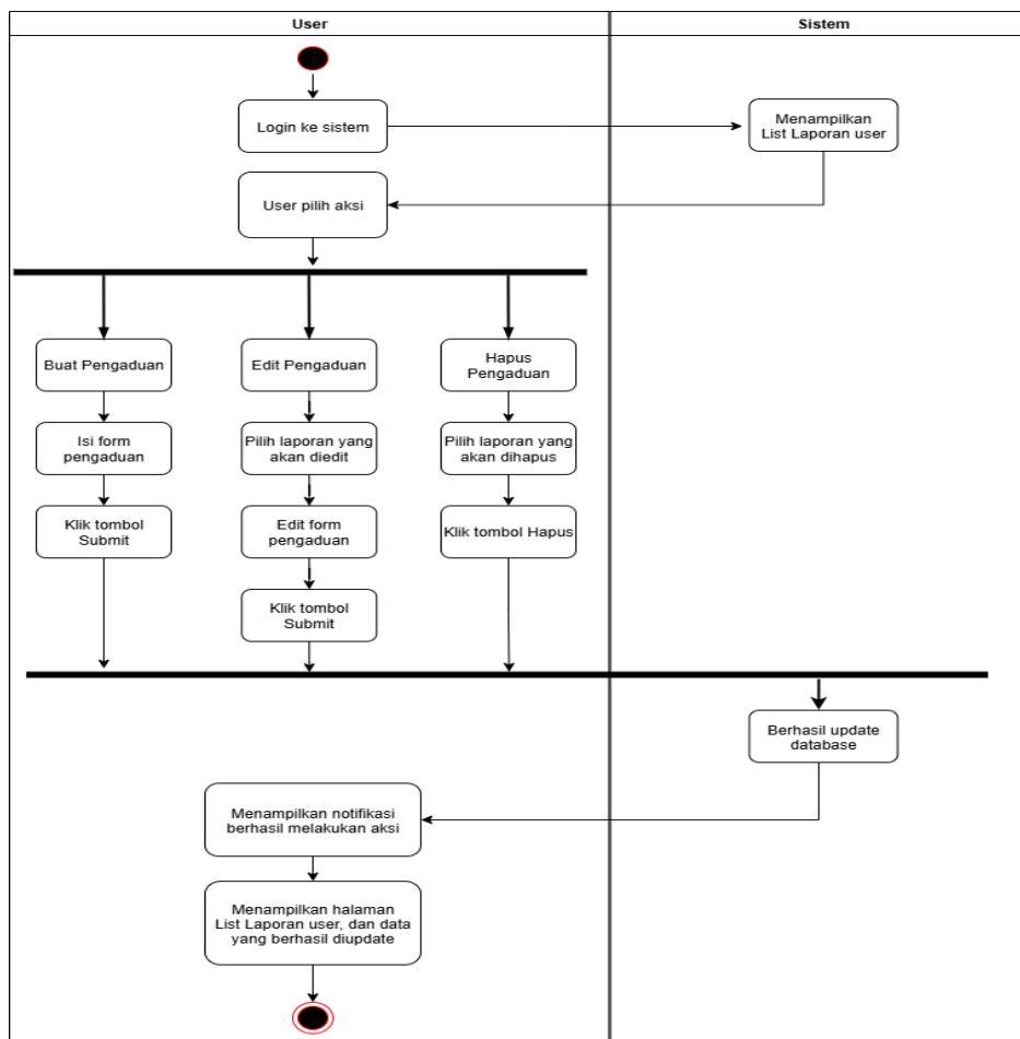
Gambar IV.4 Activity Diagram Kelola Pengaduan
