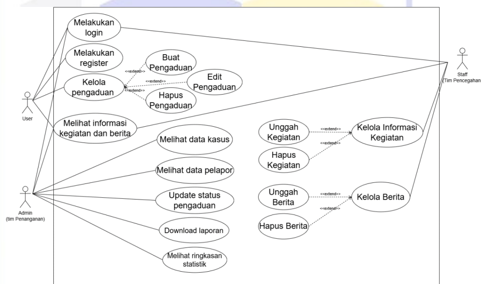
Gambar IV.1 Use Case Diagram
