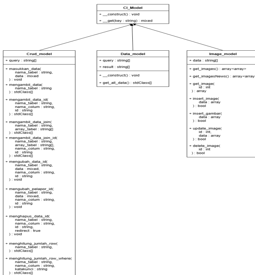
Gambar IV.14 Class Diagram CI_Model
