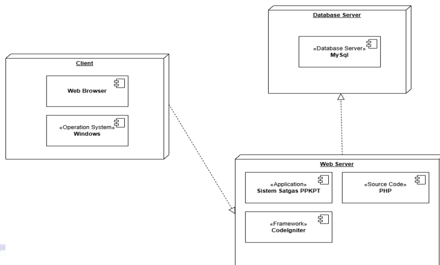
Gambar IV.35 Deployment Diagram Sistem Web Satgas PPKPT
