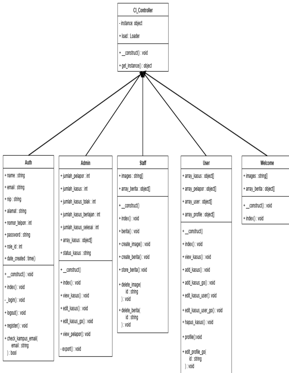
Gambar IV.13 Class Diagram CI_Controller
