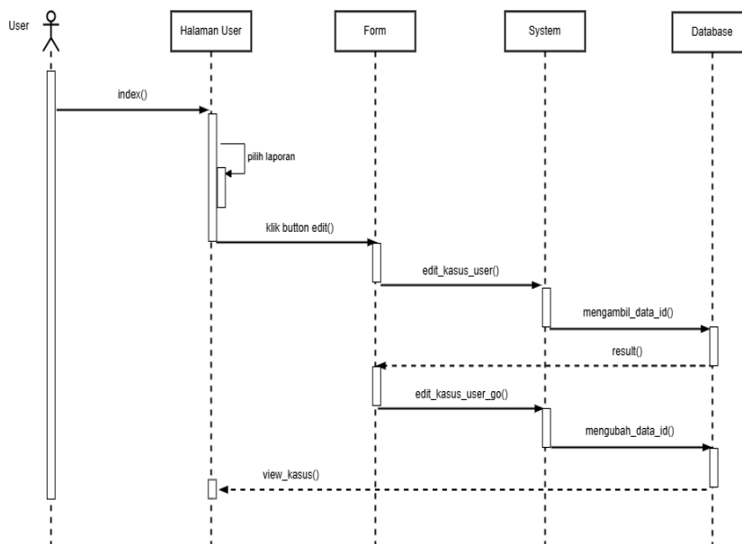
Gambar IV.18 Sequence Diagram User Edit Pengaduan
