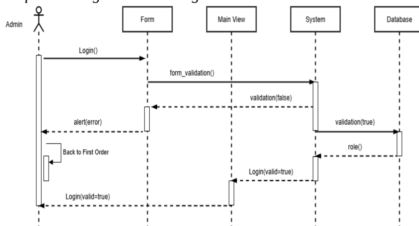
Gambar IV.21 Sequence Diagram Admin Login
