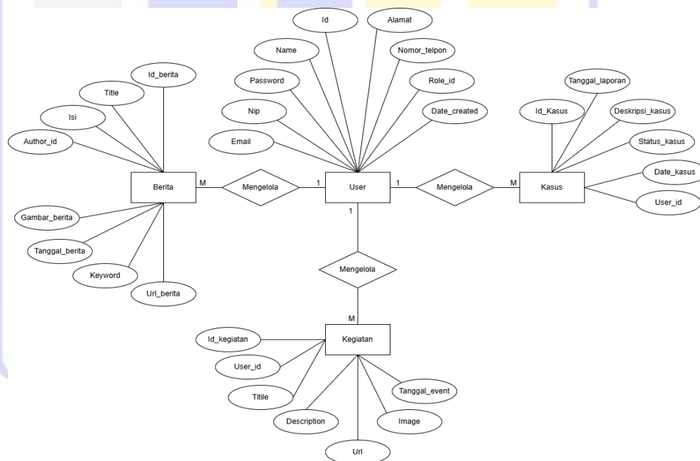
Gambar IV.36 Entity Relation Diagram model Chen's
