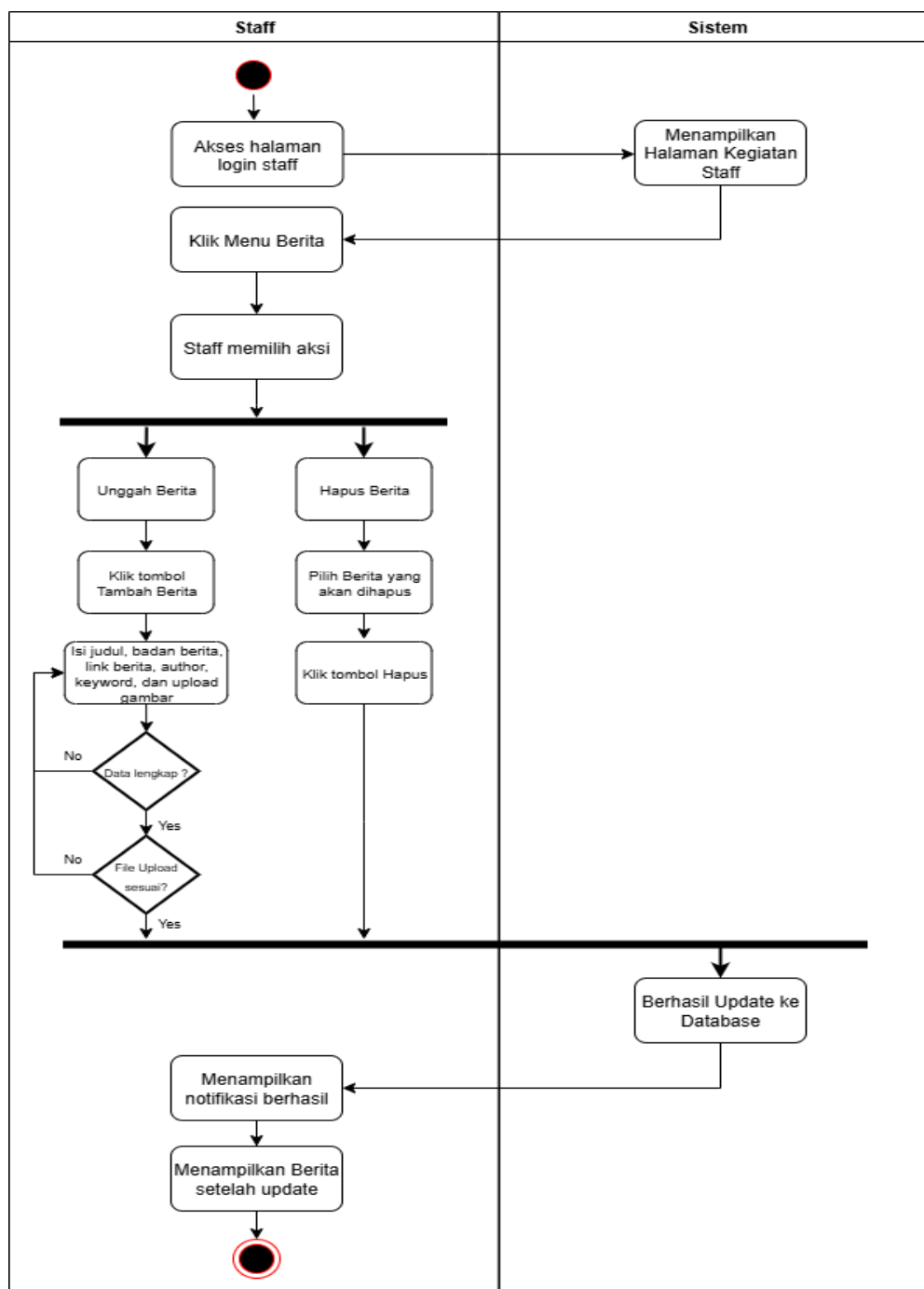
Gambar IV.12 Activity Diagram Kelola Berita
