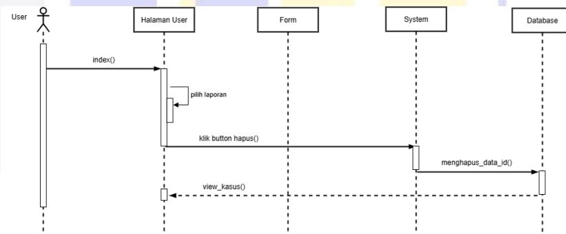
Gambar IV.19 Sequence Diagram User Menghapus Pengaduan
