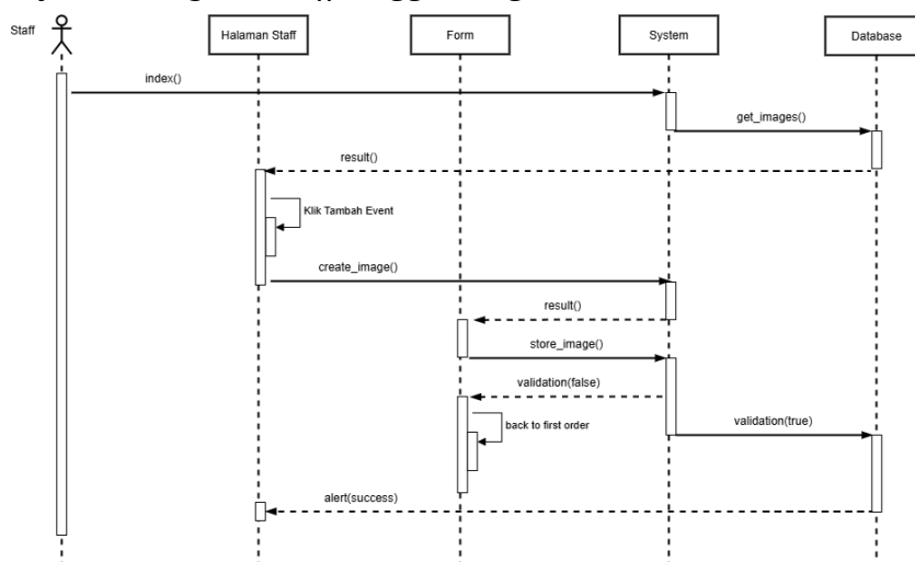
Gambar IV.30 Sequence Diagram Staff Unggah Kegiatan
