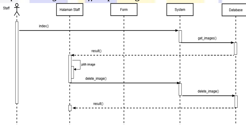
Gambar IV.31 Sequence Diagram Staff Hapus Kegiatan
