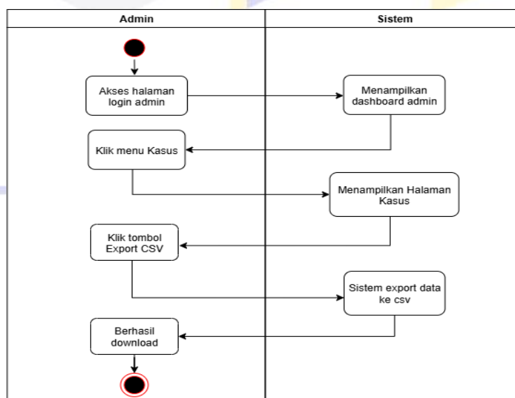
Gambar IV.9 Activity Diagram Download Laporan
