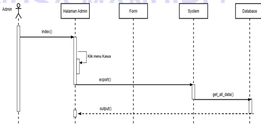
Gambar IV.26 Sequence Diagram Admin Download Laporan
