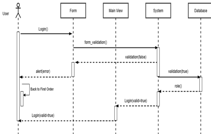
Gambar IV.16 Sequence Diagram Login
