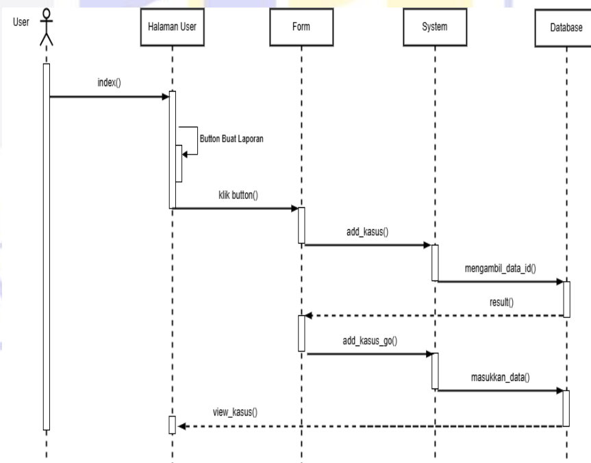
Gambar IV.17 Sequence Diagram User Buat Pengaduan
