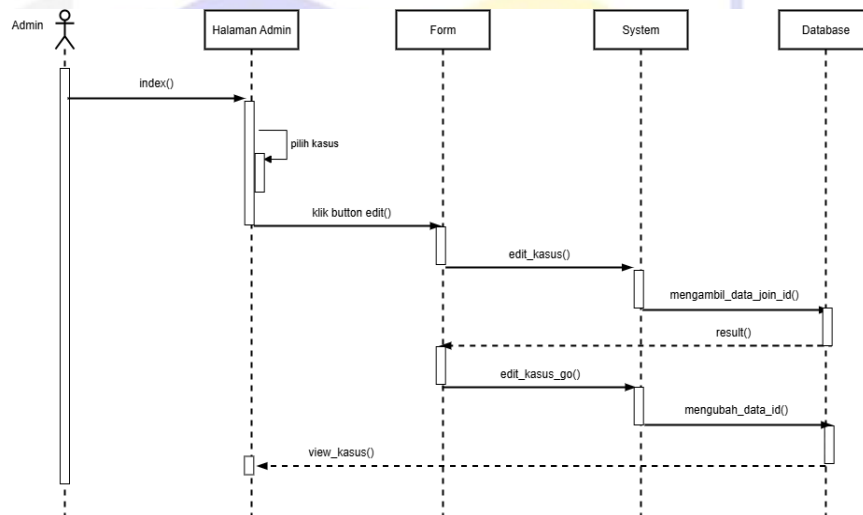
Gambar IV.25 Sequence Diagram Admin Update Status Pengaduan
