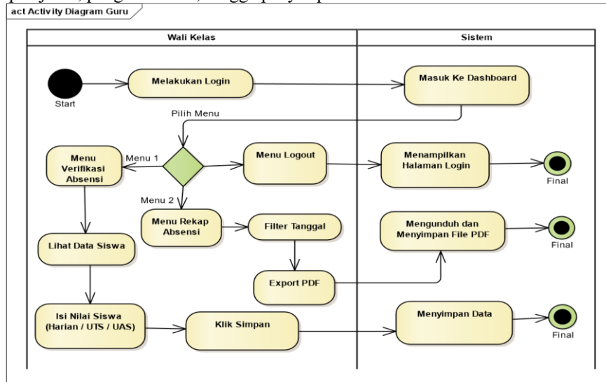
Gambar 2 Activity Diagram Proses Input Nilai
