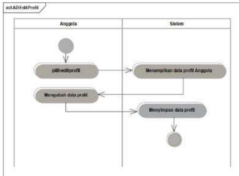
Gambar 11. Activity Diagram Ubah Profil
