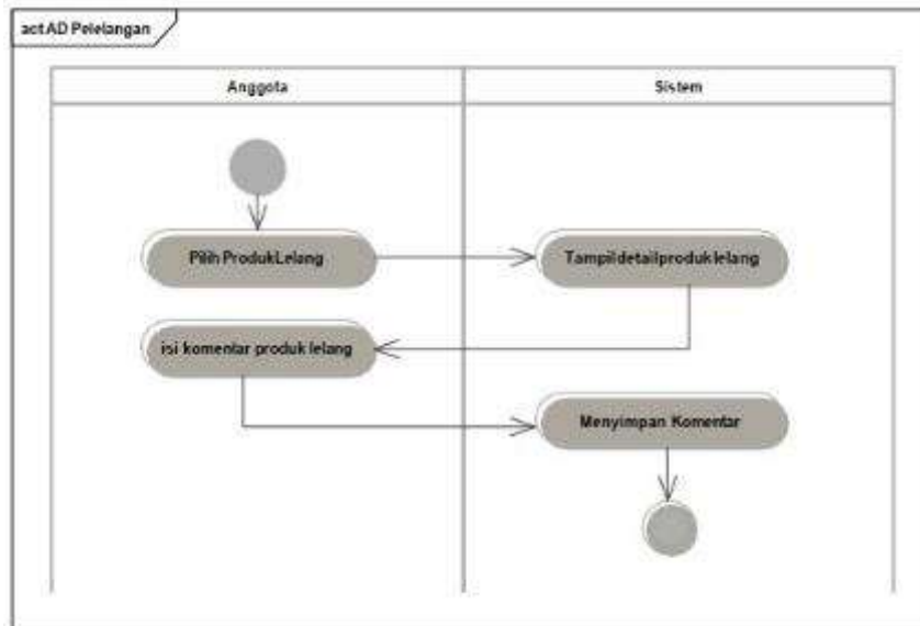
Gambar 9. Activity Diagram Pelelangan
