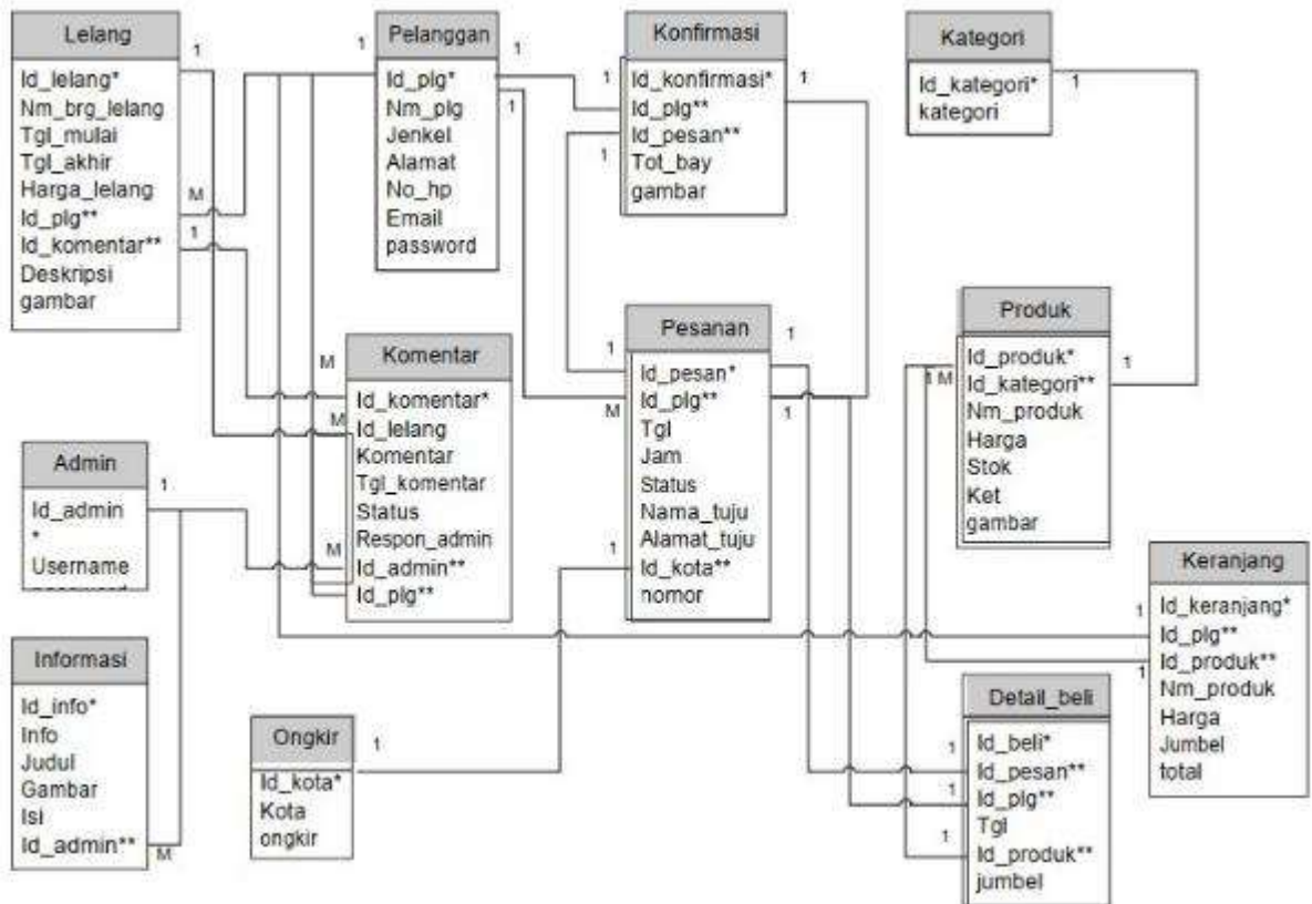
Gambar 2. Logical Record Structure D.
