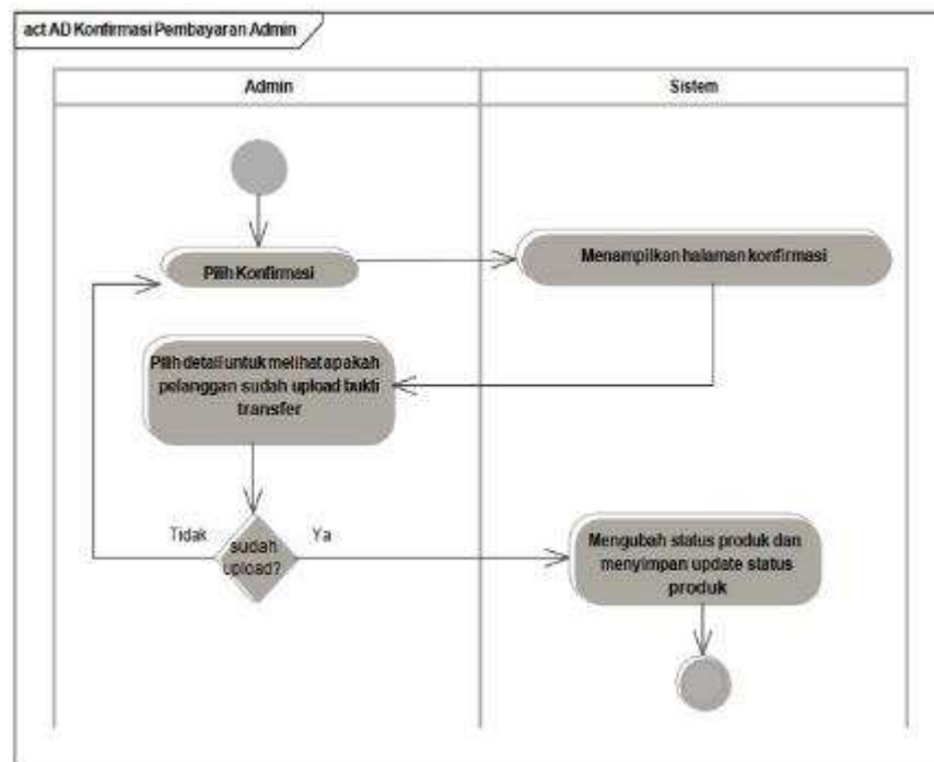
Gambar 18 Activity Diagram Kelola Transaksi
