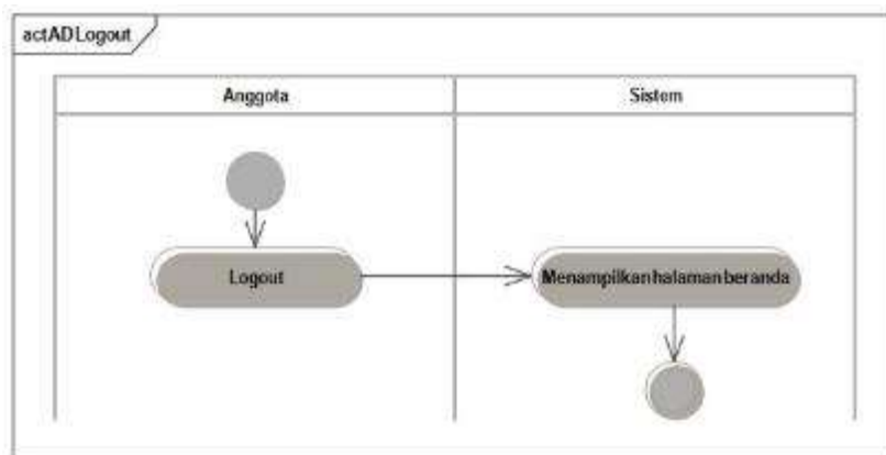
Gambar 12. Activity Diagram Logout Anggota
