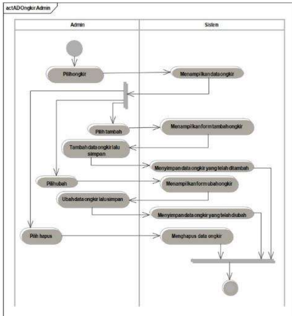
Gambar 16. Activity Diagram Kelola Ongkir
