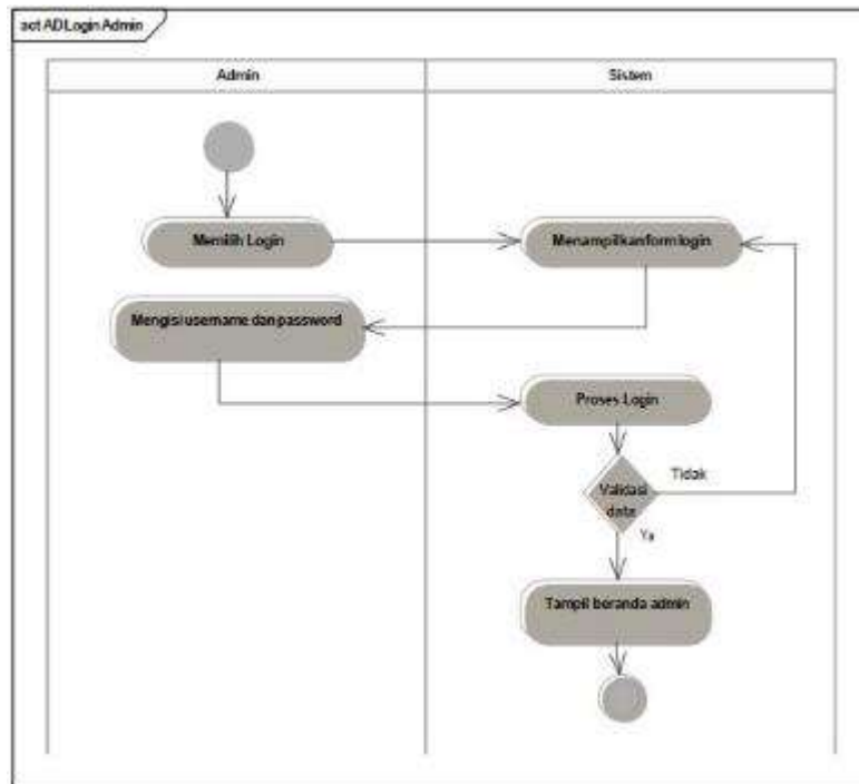
Gambar 13. Activity Diagram Login Admin
