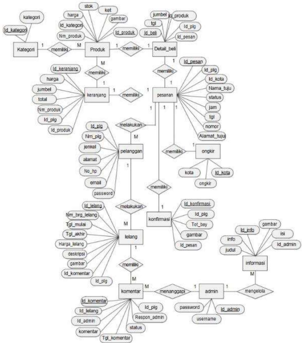
Gambar 1. Entity Relationship Diagram
