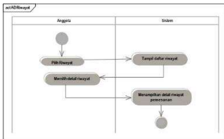
Gambar 10. Activity Diagram Cek Riwayat Pembelian
