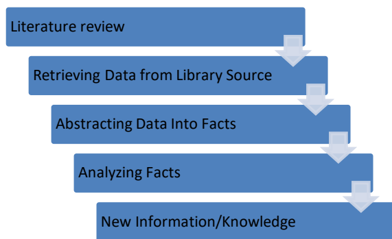
Figure 1. Framework Literature
