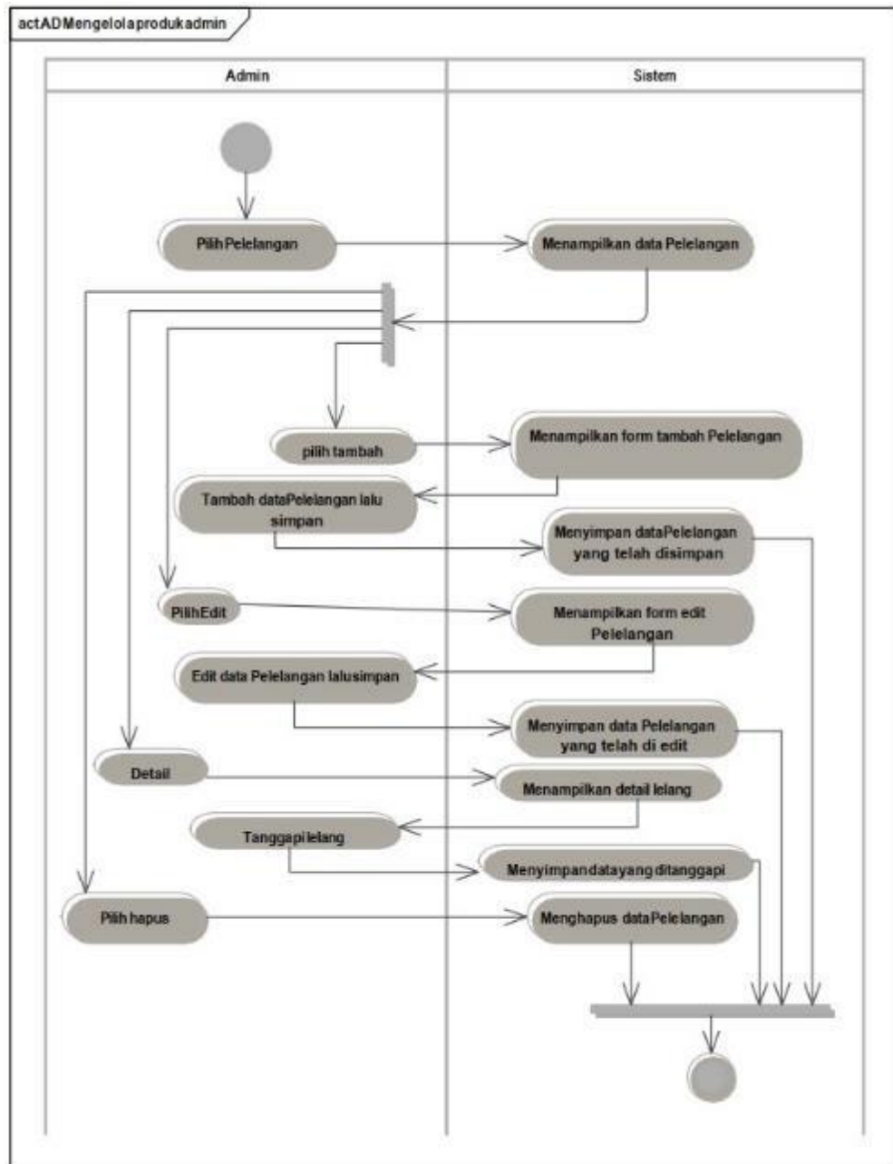
Gambar 15. Activity Diagram Kelola Pelelangan
