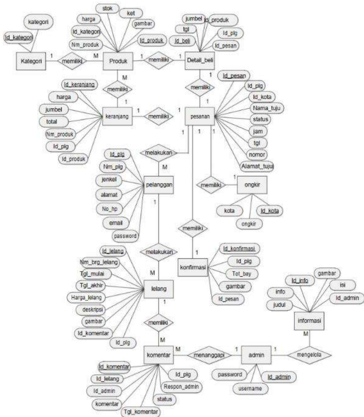
Gambar 1. Entity Relationship Diagram
