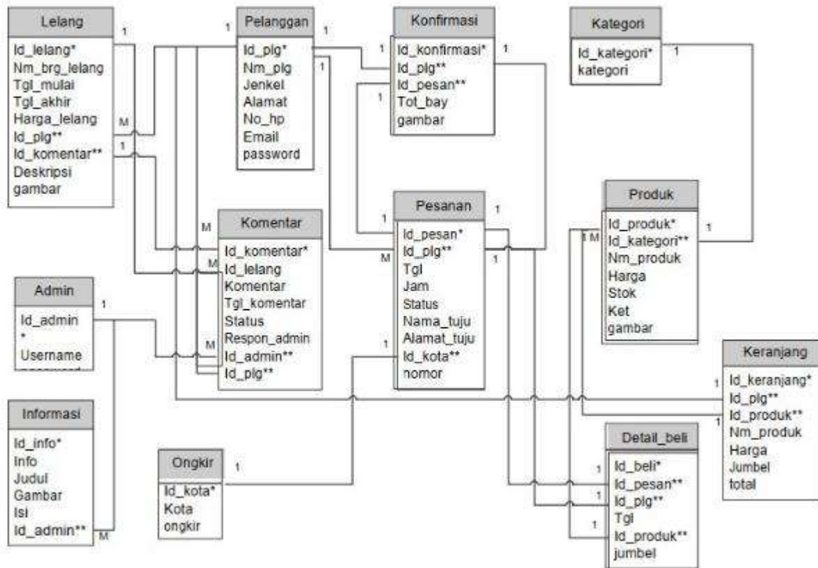
Gambar 2. Logical Record Structure
