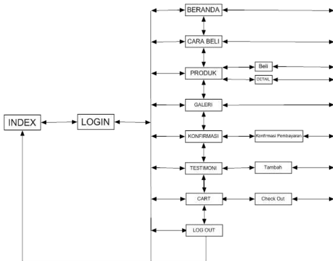
Gambar III.7. Struktur Navigasi Halaman Member
