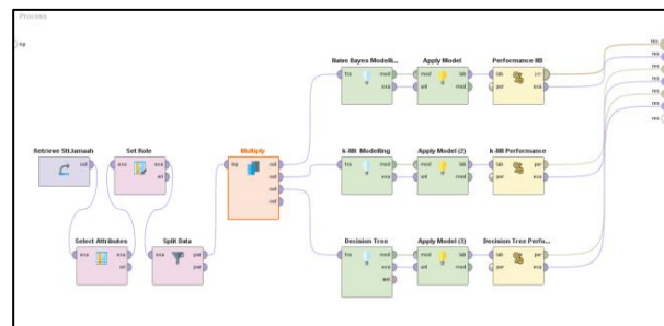
Figure 4. Naïve Bayes, k-NN and Decision Tree Algorithm Modeling
