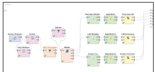
Figure 5. Modeling of Naïve Bayes, k-NN and Decision Tree algorithms using the SMOTE data balancing method
