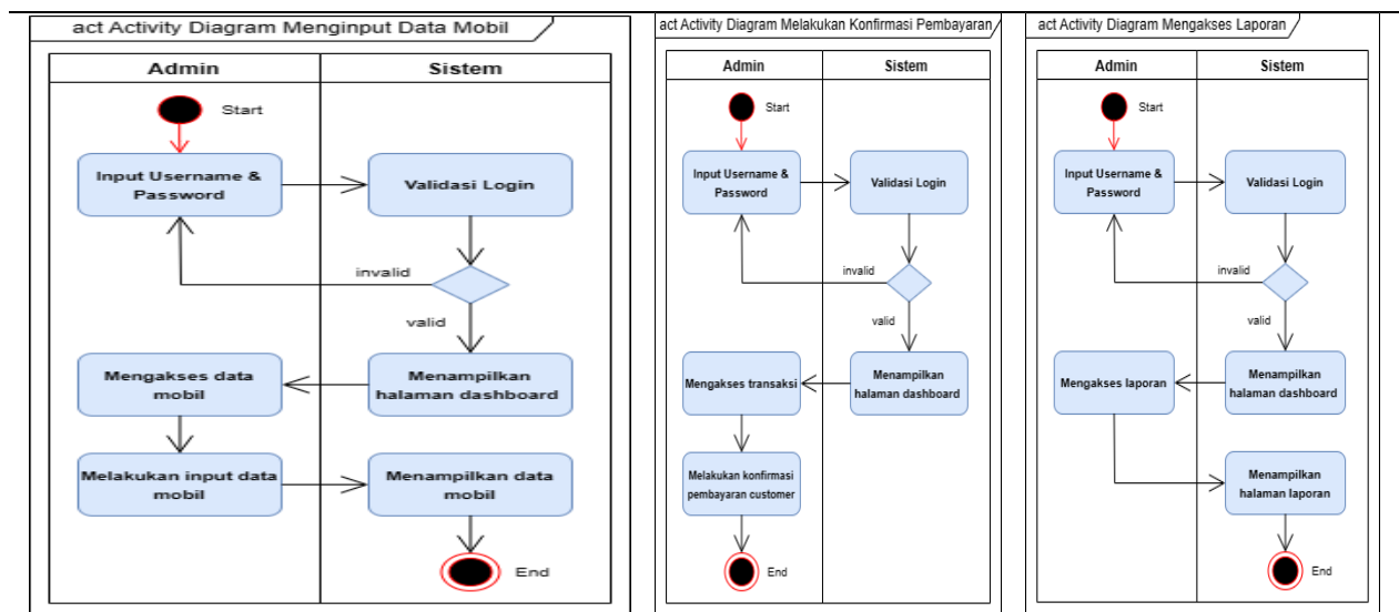
Gambar 3. Activity Diagram Admin
