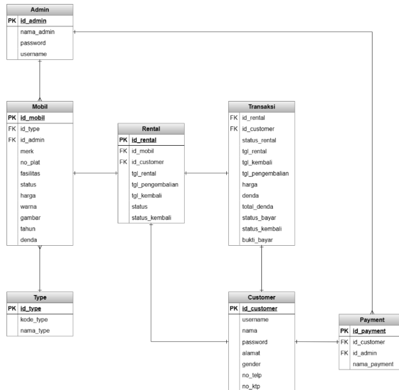
Gambar 5. Logical Record Structure (LRS)
