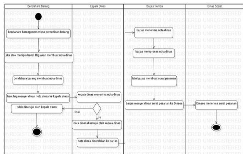
Gambar 2 Activity Diagram proses permintaan
