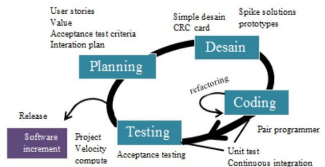
Gambar 1. Tahapan Model XP Sumber: (Ariyanti et al., 2020)
