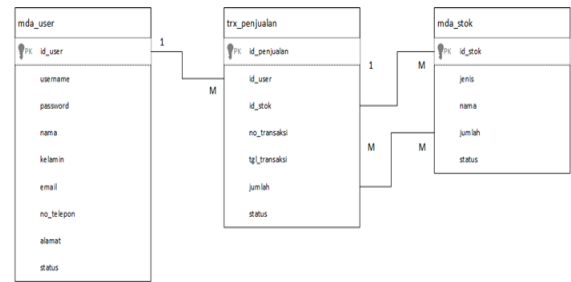
Gambar 8. Logical Record Structure Diagram
