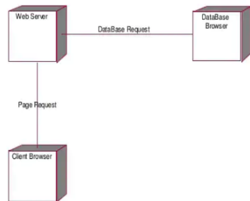
Gambar 9. Deployment Diagram
