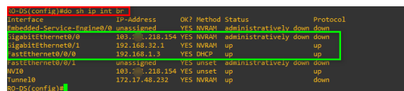
Gambar 11. Status Interface GigabitEthernet0/0
