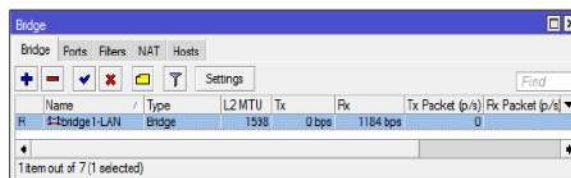
Gambar 6. Menu Bridge
