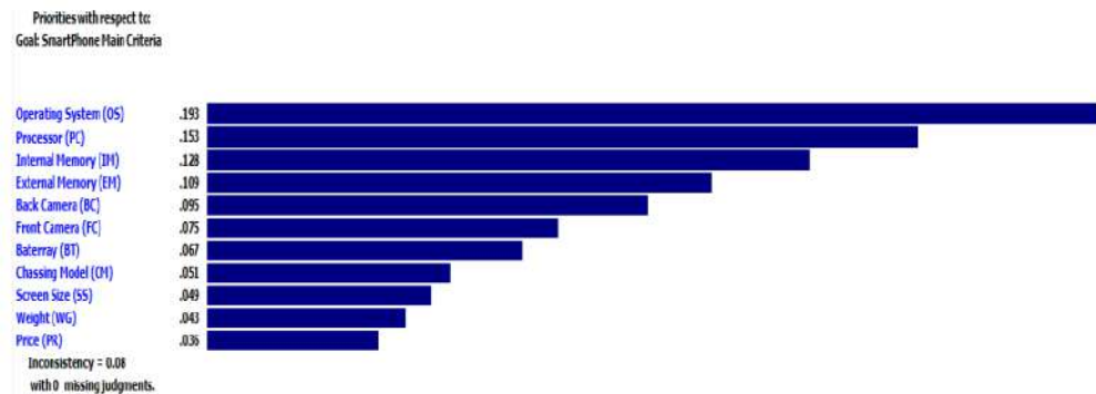
Fig. 2. Synthesis of eigenvector using expert choice apps.
