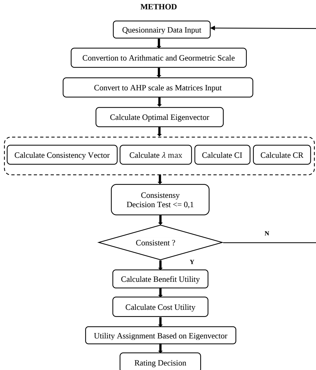
Fig. 1. AHP-SMART Algorithm
