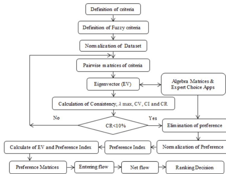
Figure 1. MCDM-AHP-PROMETHEE algorithm
