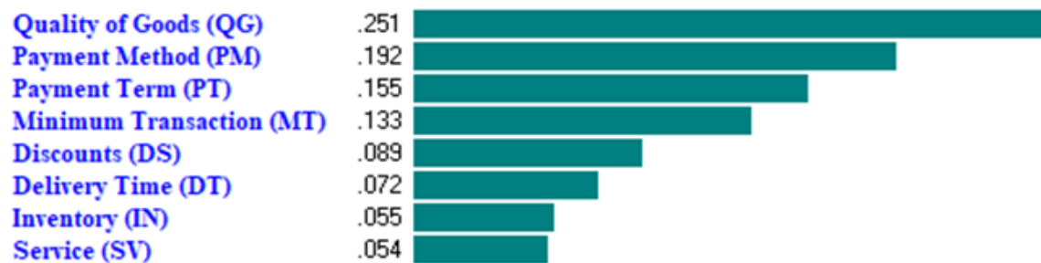
Figure 2. Synthesis of eigenvector using expert choice apps
