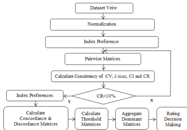
Figure 1. AHP-ELECTRE Algorithm
