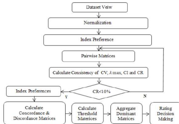
Figure 1. AHP-ELECTRE Algorithm
