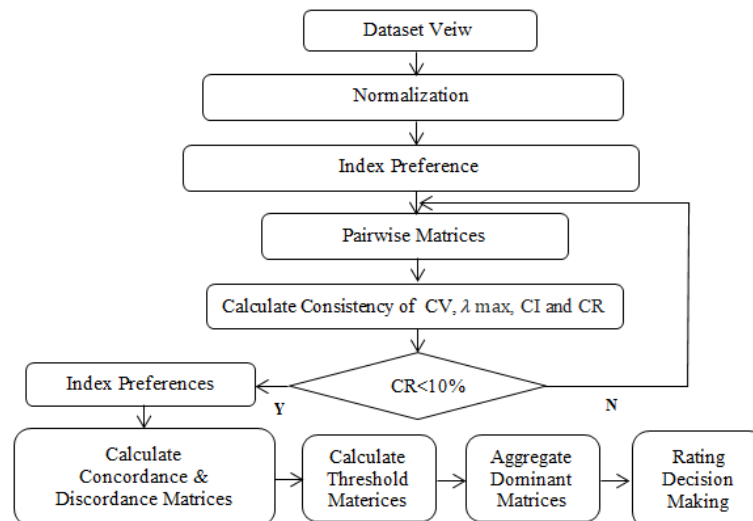
Figure 1. AHP-ELECTRE algorithm
