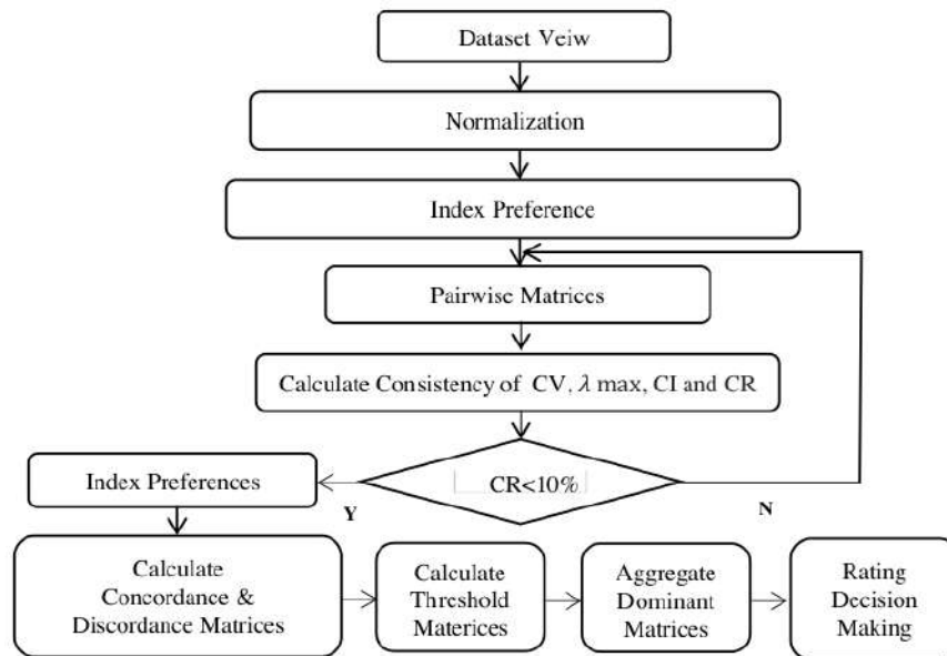
Fig. 2. AHP-ELECTRE Algorithm
