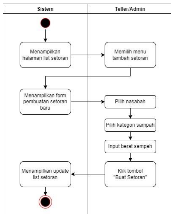
Gambar 3. Activity Diagram Setoran Sampah
