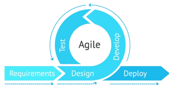
Gambar 1. Metode Agile
