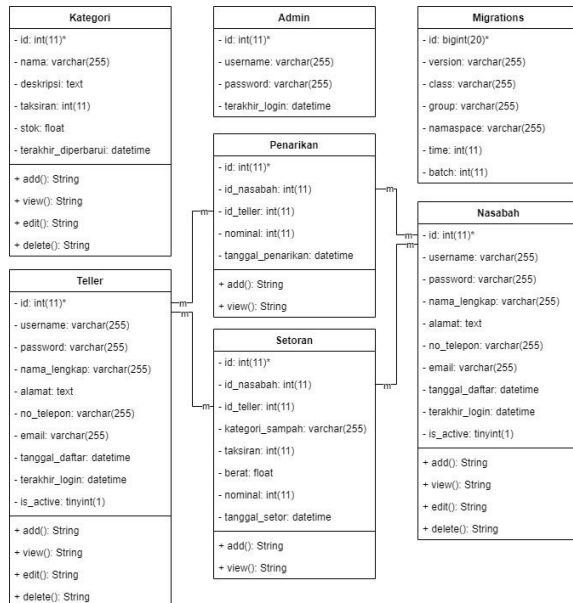
Gambar 5. Class Diagram
