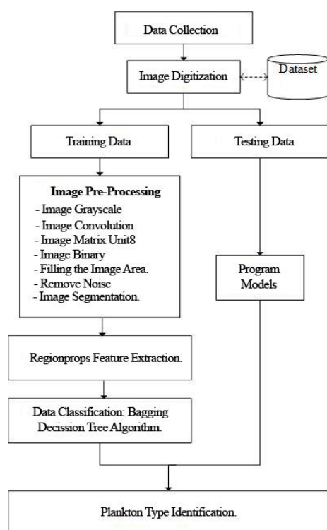
Figure 1. Research Model
