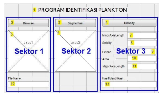
Figure 14. Program Design
