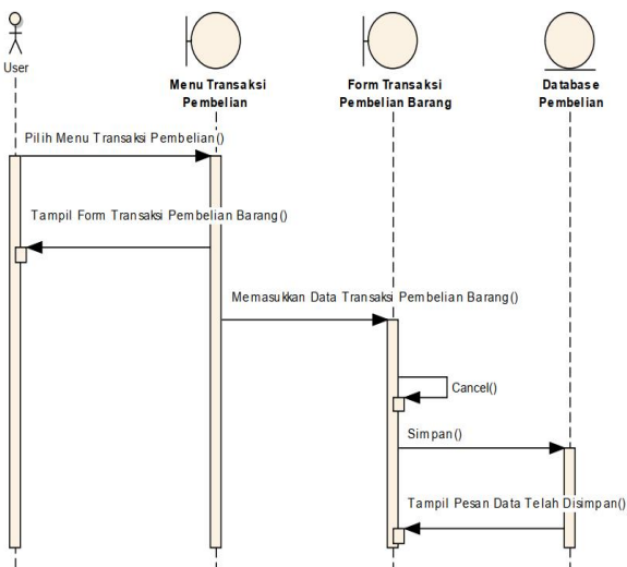
Gbr 17. Sequence Diagram Pembelian
