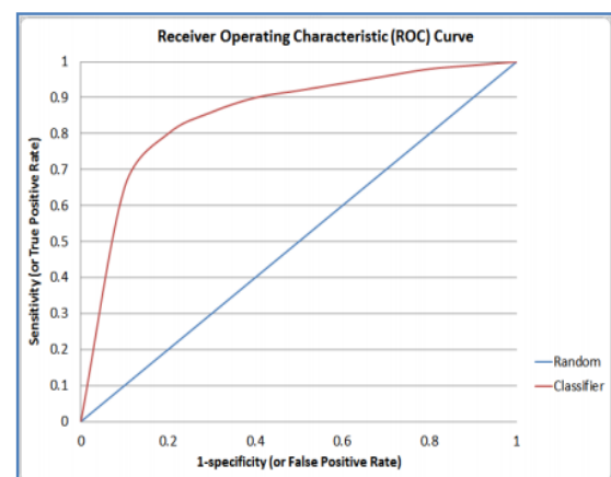
Gambar 4. ROC curve
