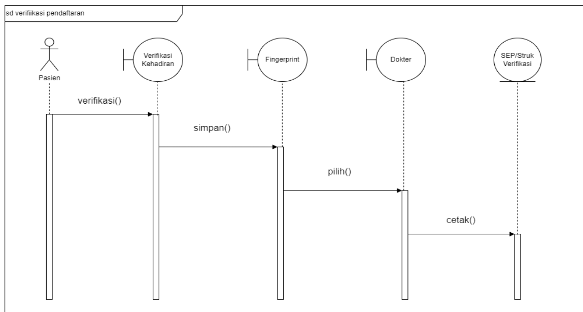
Gambar 4. Sequence Diagram Pendaftaran
