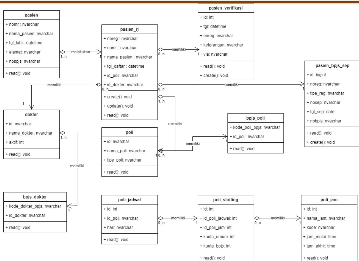
Gambar 3. Class Diagram
