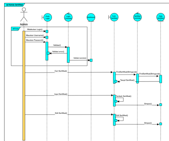
Figure 8 Sequence Diagram
