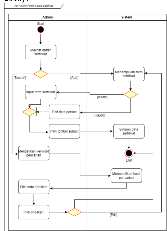
Figure 4 Activity Diagram
