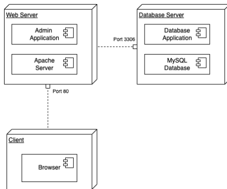
Figure 10 Deployment Diagram
