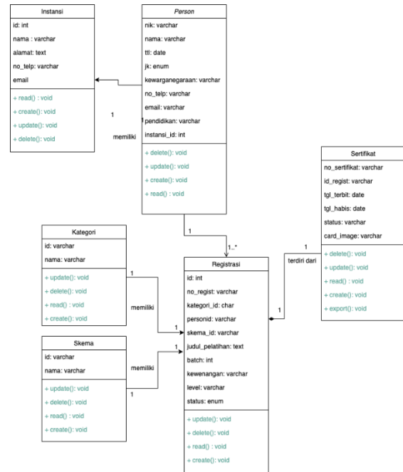
Figure 7 Class Diagram
