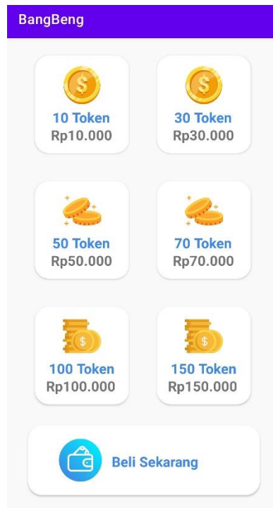
Gambar 12. Halaman TopUp
