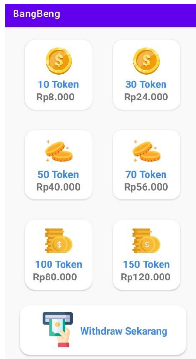
Gambar 13. Halaman Withdraw
