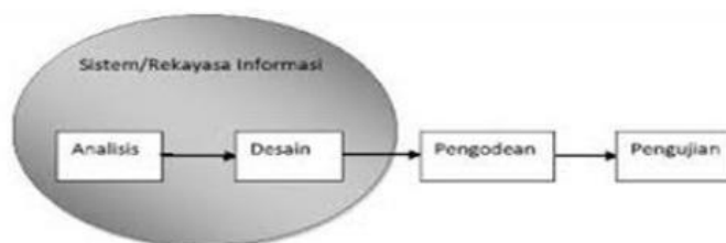
Gambar 1. Model Waterfall
