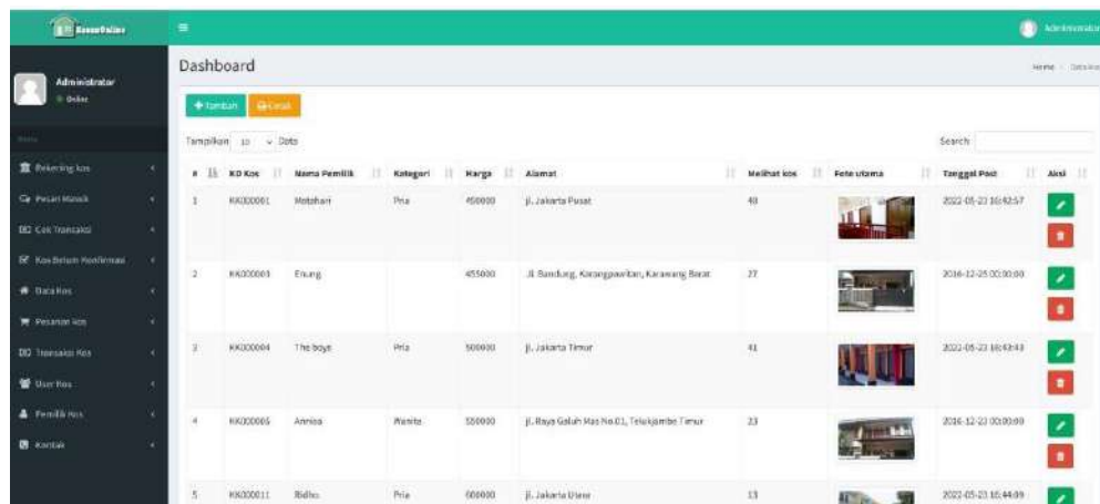
Gambar 10. Gambar Dashboard
