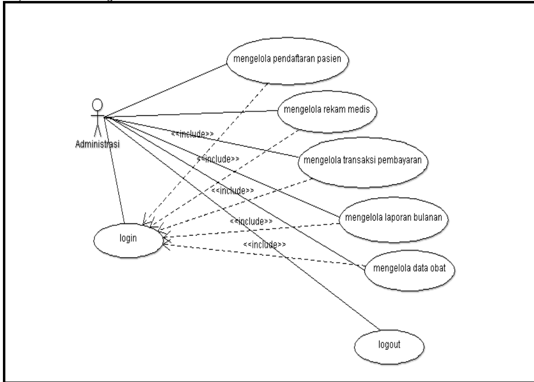
Gambar 1 Use Case Diagram Administrasi
