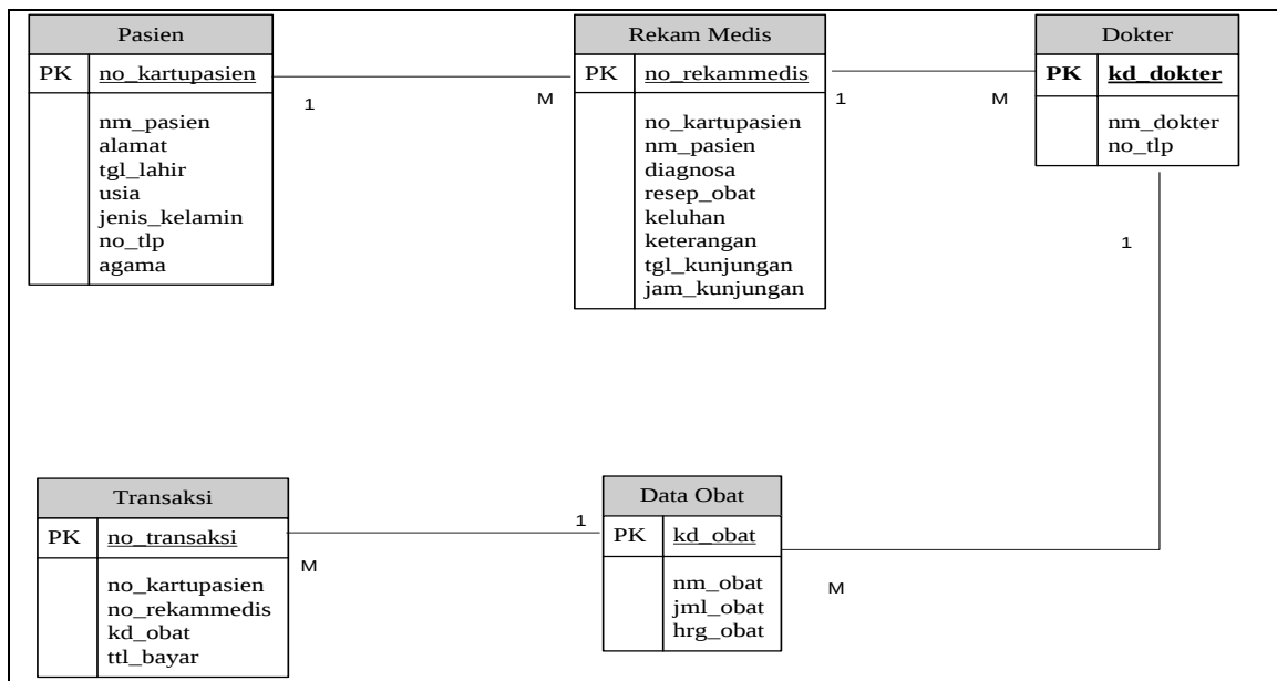
Gambar 7 Logical Record Structure (LRS)
