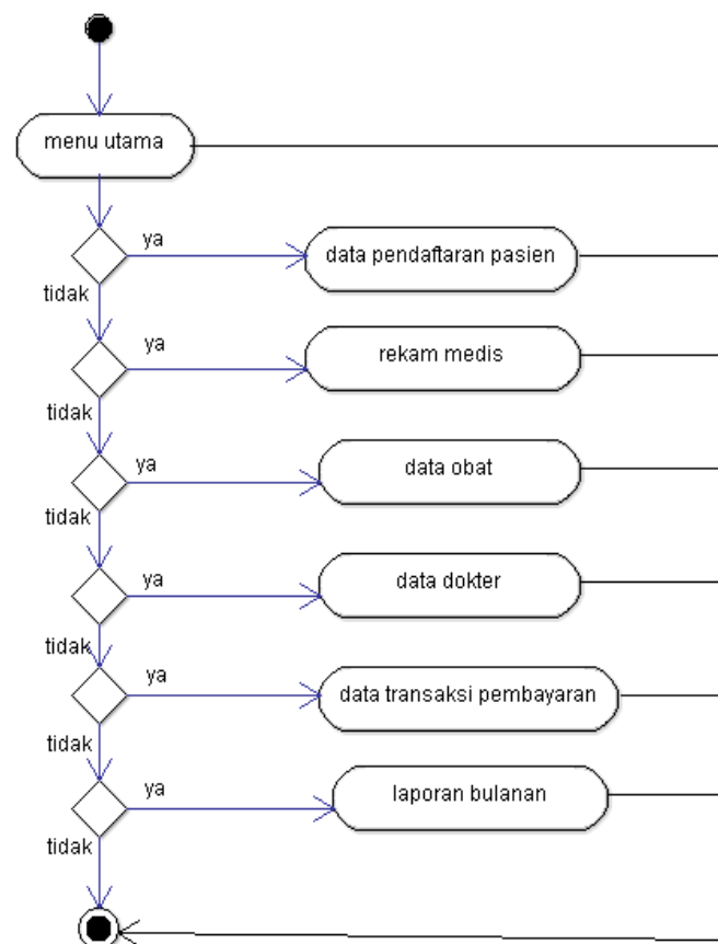
Gambar 5 Activity diagram Menu Utama
