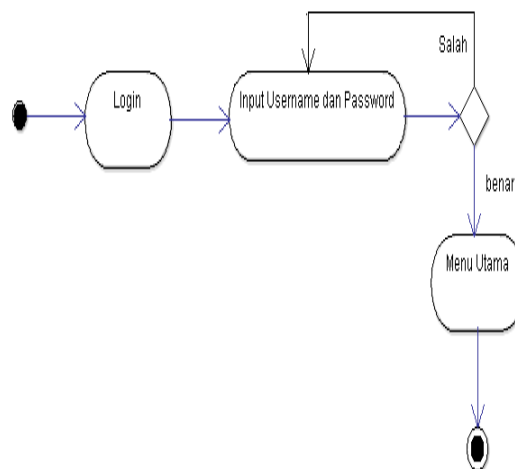
Gambar 4 Activity diagram halaman login
