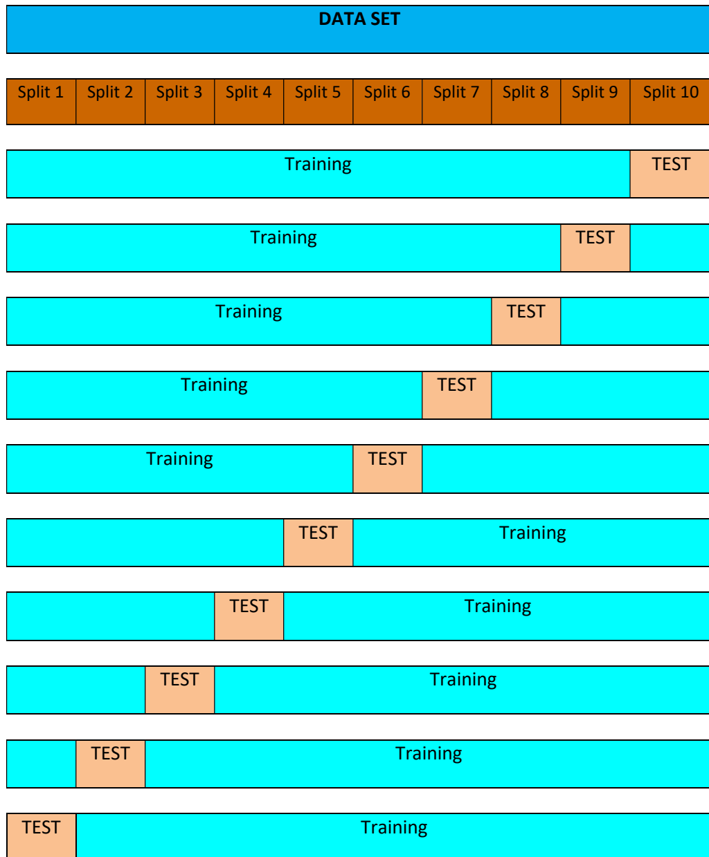
Gambar 2.2 Ilustrasi 10 Fold Cross Validation
