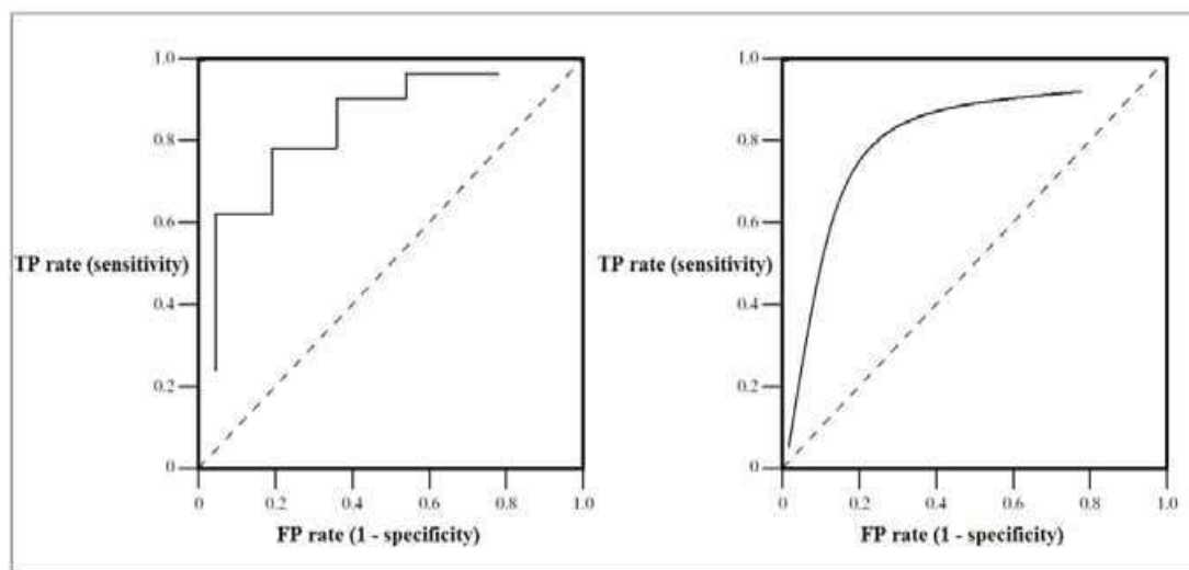
Gambar 2.3 Grafik ROC ( discrete dan continuous ) (Gorunescu, 2011)
