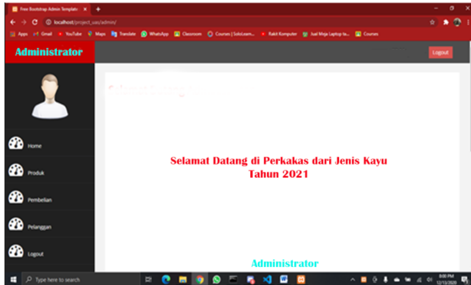
Gambar 1. Layar Administrator
