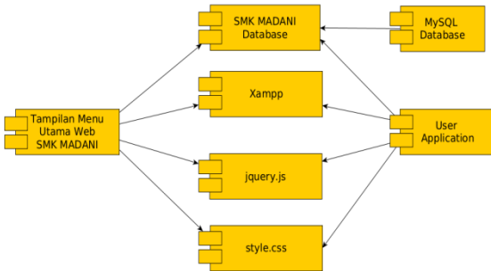
Gambar 8. Component diagram
