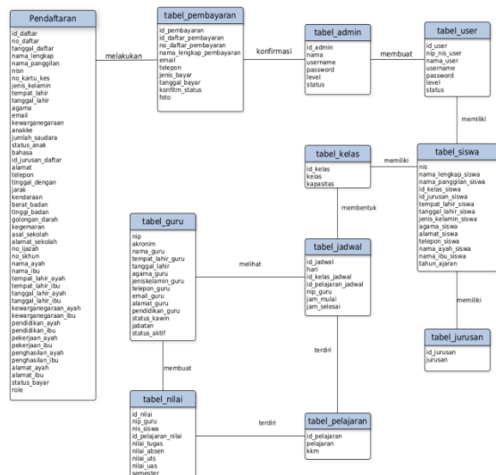
Gambar 6. Logical data model
