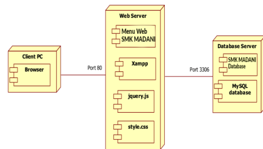
Gambar 9. Deployment diagram
