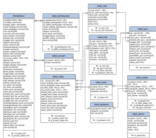
Gambar 7. Physical data model
