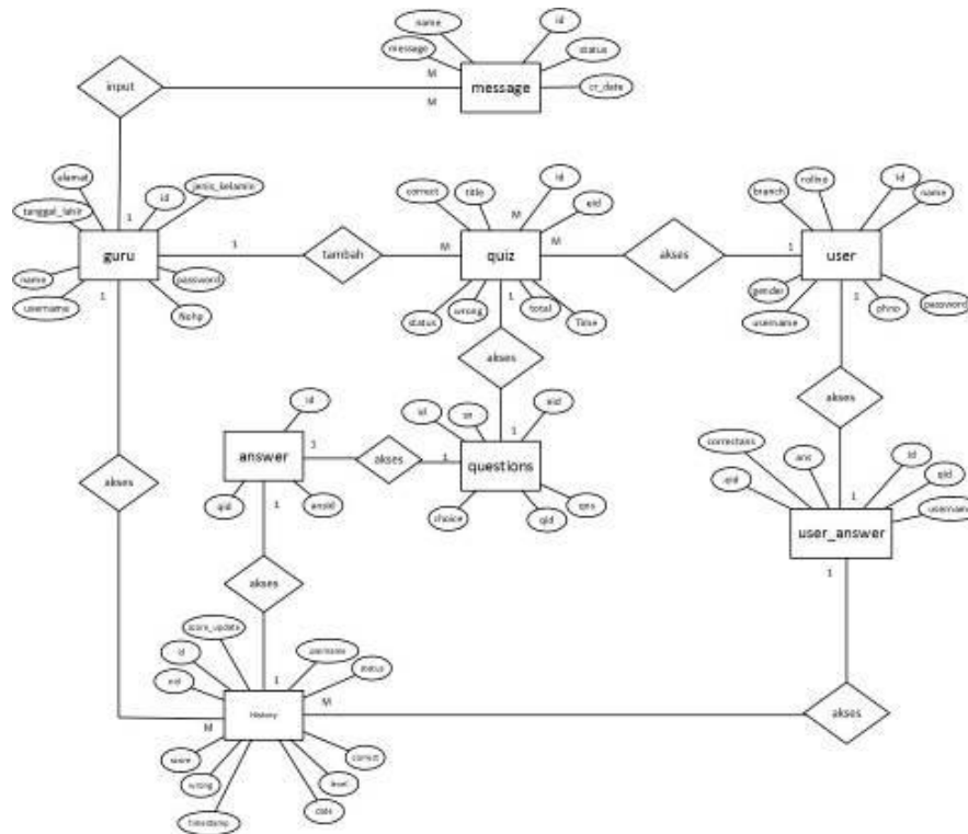
Gambar 7. Tampilan Entity Relationship Diagram (ERD)
