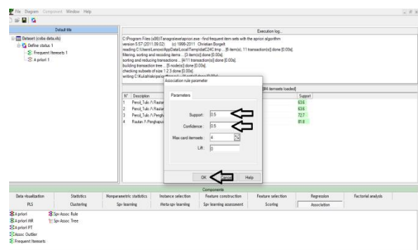
Figure 4. The Process of Determining Minimum Support and Minimum Confidence
