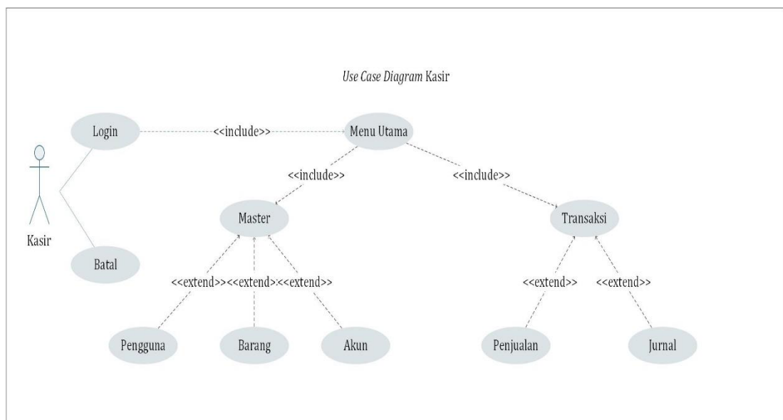
Gambar 1. Use Case Diagram Kasir
