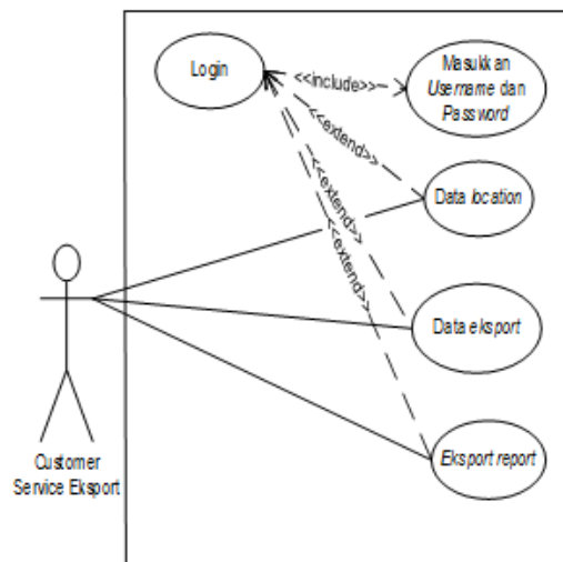
Gambar 3. Use case Diagram Halaman Bagian Customer Service Ekspor
