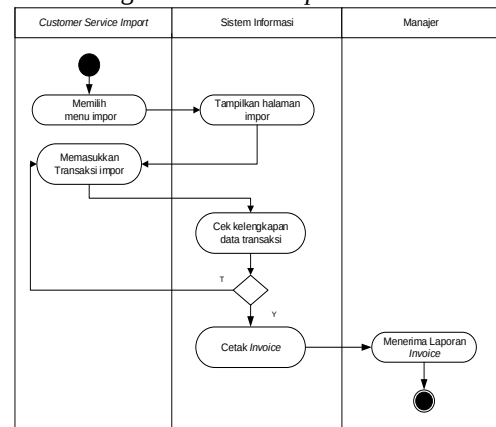
Gambar 5. Activity Diagram Transaksi Import
