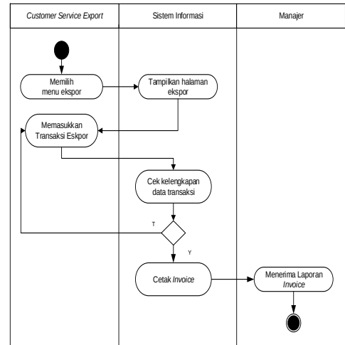
Gambar 4. Activity Diagram Transaksi export
