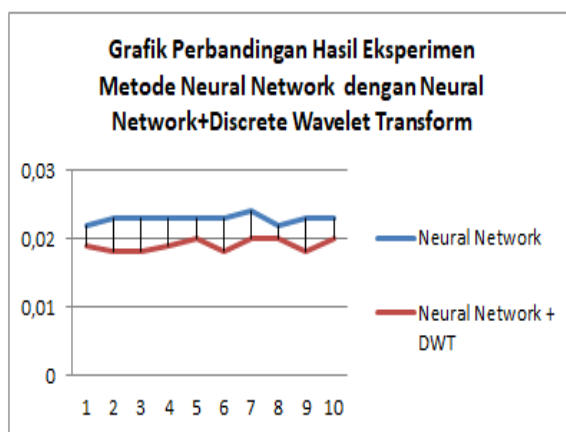
Gambar 4. Grafik Perbandingan RMSE Neural Network (Fungsi Aktivasi Binary Sigmoid dan Neural Network (Fungsi Aktivasi Binary Sigmoid )+ Discrete Wavelet Transform
