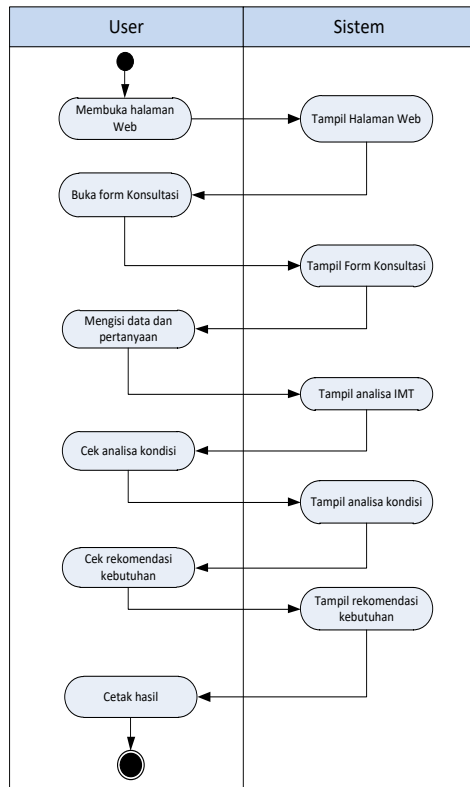
Sumber: (Ariesaputra & Sihombing, 2019) Gambar 5. Activity Diagram Konsultasi User
