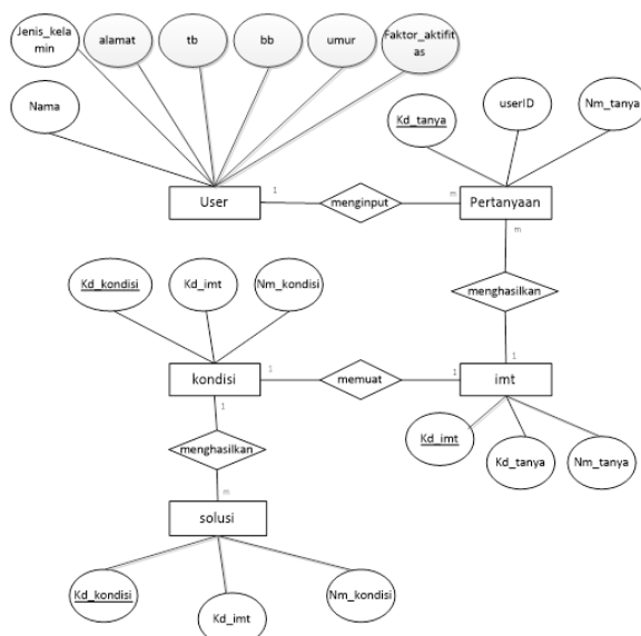
Sumber: (Ariesaputra & Sihombing, 2019) Gambar 6. Entity Relationship Diagram Sistem Pakar Pedoman Kalkulasi Gizi Seimbang
