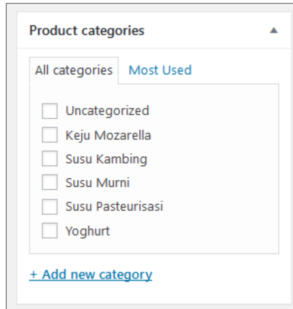
Gambar 36. Product category.
