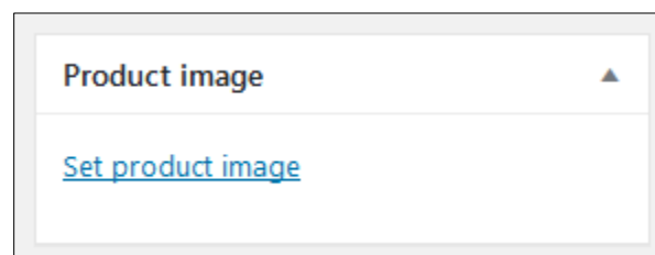
Gambar 37. Product image.
