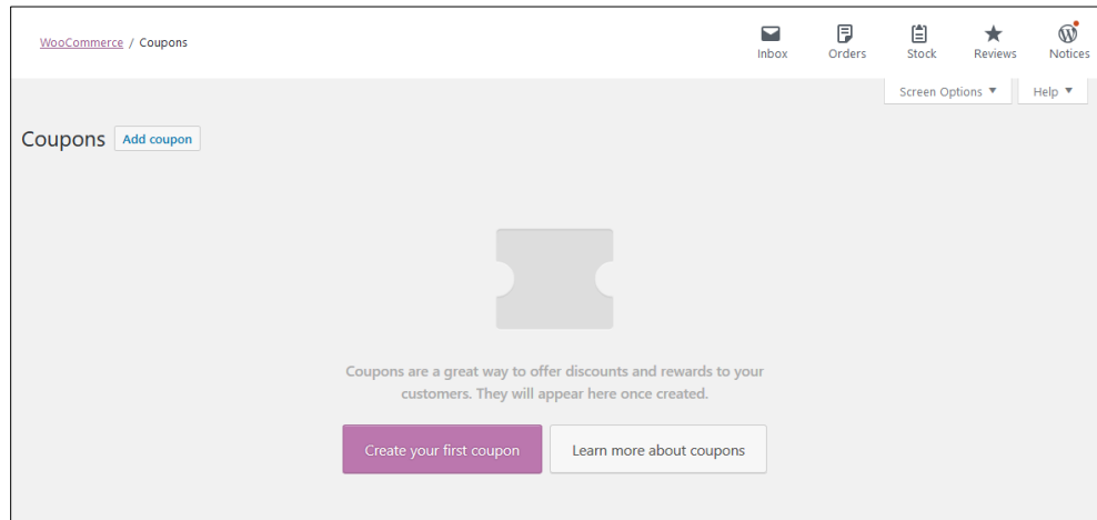
Gambar 19. Coupons.
