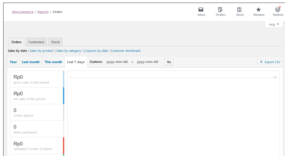
Gambar 20. Reports.
