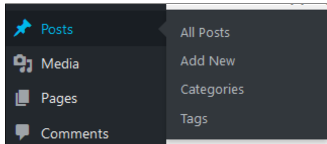
Gambar 12. Posts.
