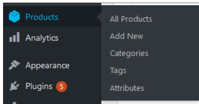
Gambar 31. Products.
