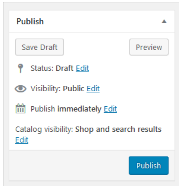
Gambar 38. Publish.
