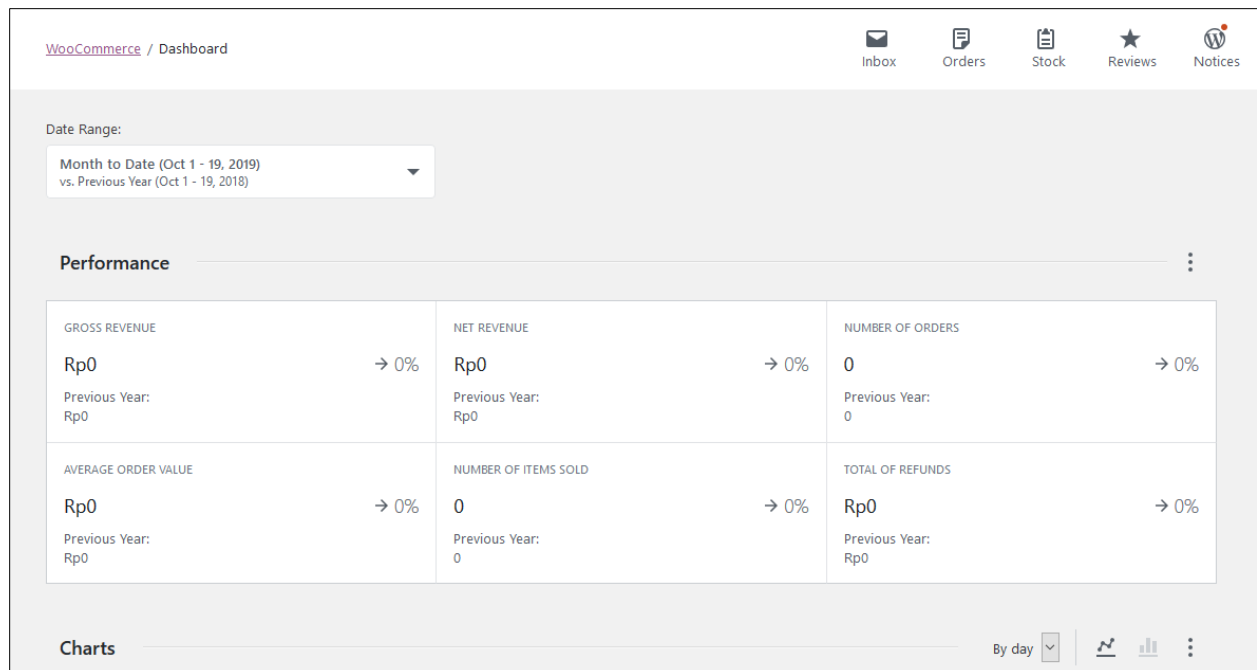
Gambar 17. Dashboard.
