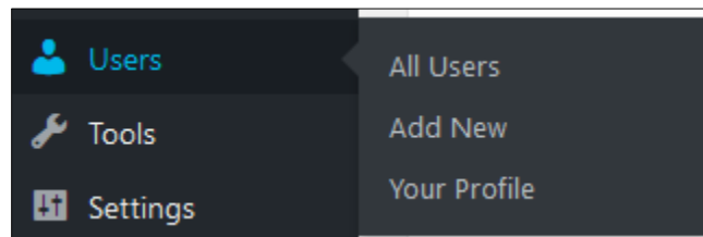
Gambar 2. Menu users.
