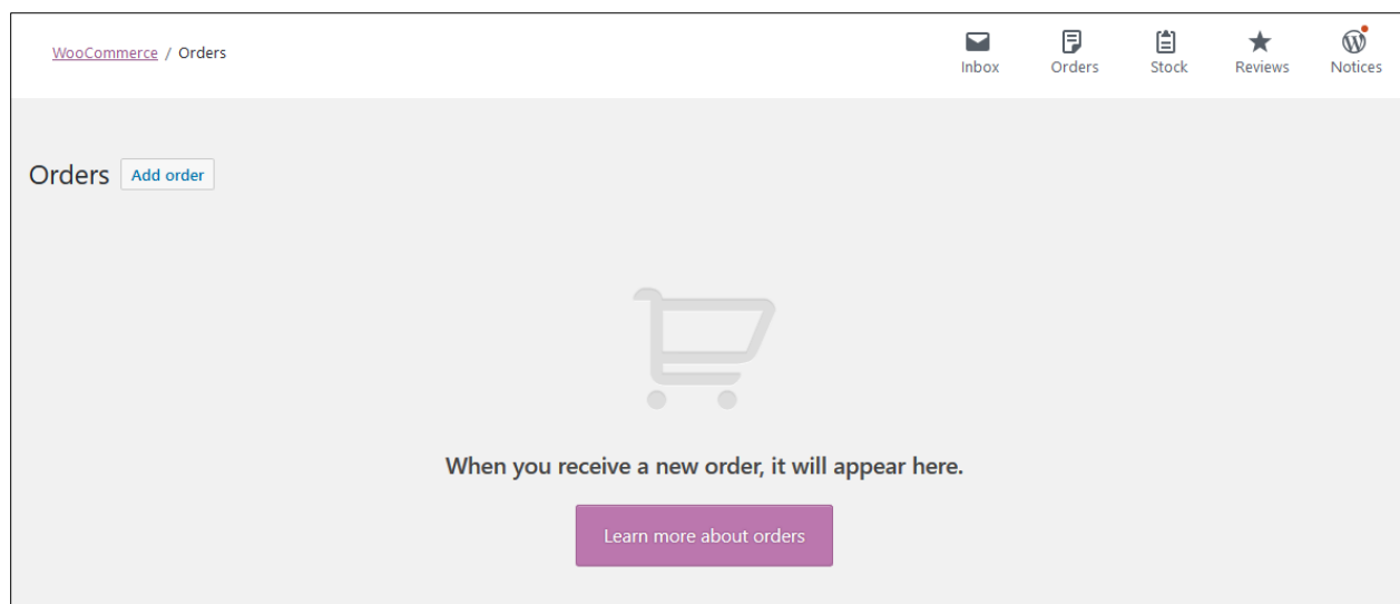
Gambar 18. Orders.
