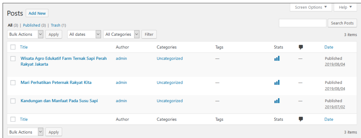
Gambar 13. All posts.
