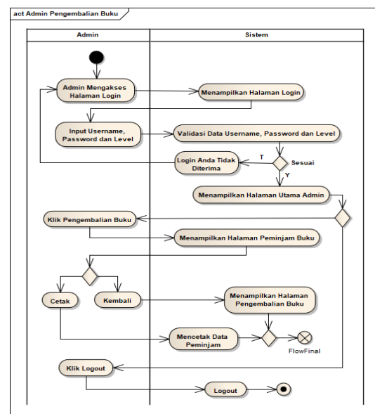
Gambar 4. Activity Diagram Pengembalian Buku
